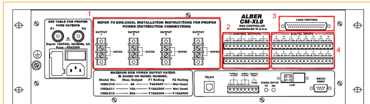
Figure 9. CM-XL8 Output/Load Control/Control Outputs/Digital Inputs
