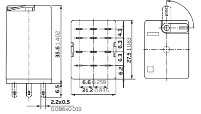
CR-M relay with 3 c/o contacts
