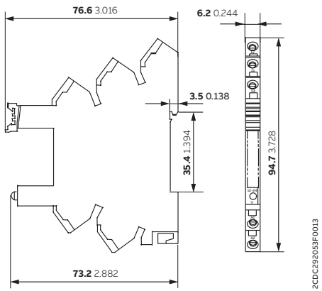
CR-S socket - spring connection
