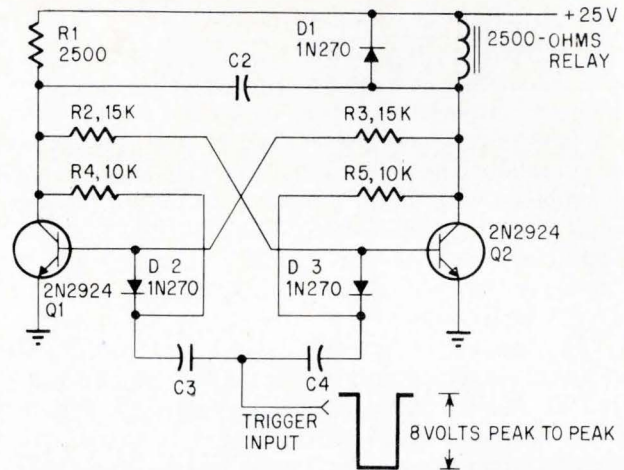
Addition of capacitor C_2 prevents accidental triggering of bistable multivibrator because of noise.
