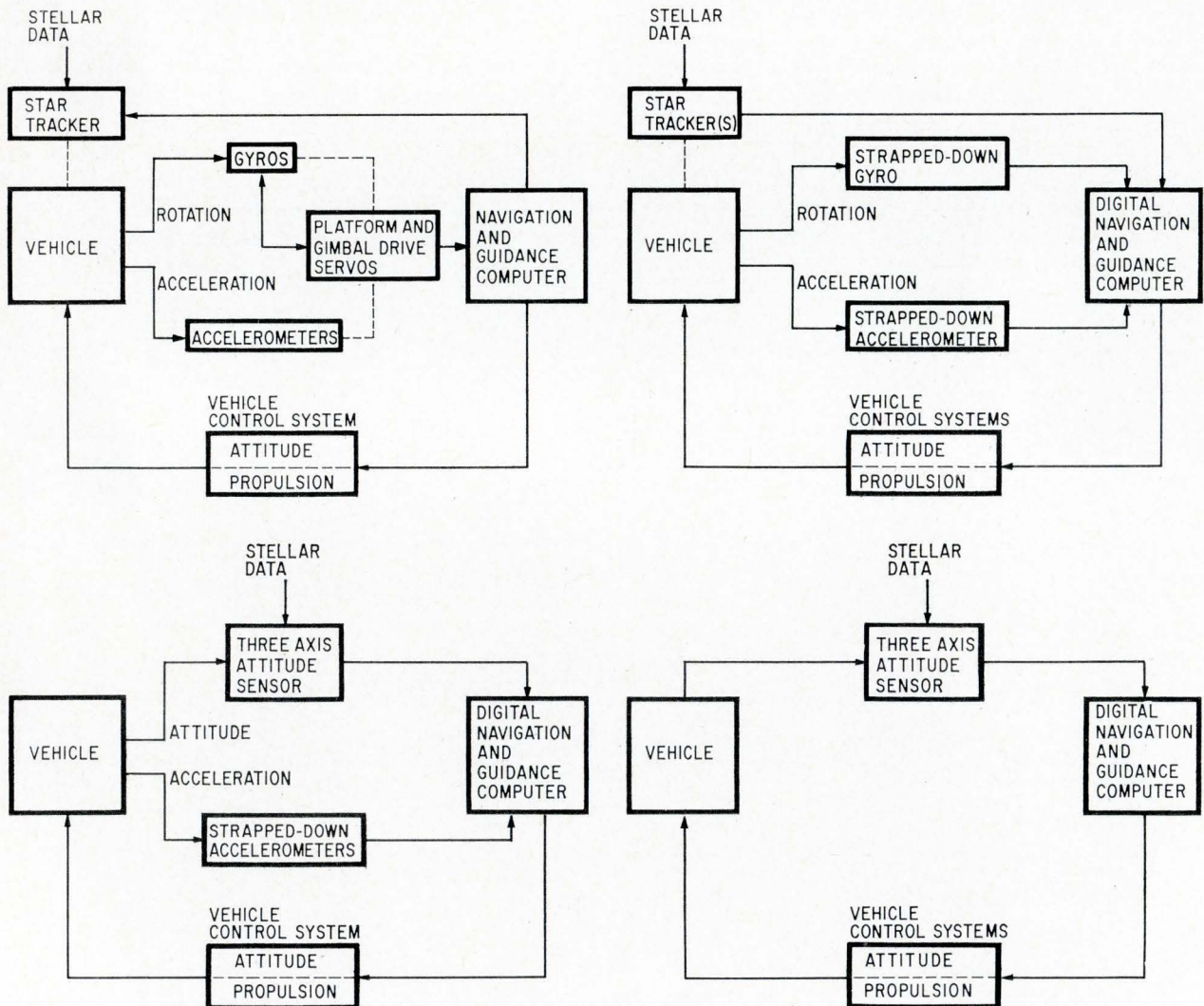
Four guidance systems. At top left, gimbals, gyroscopes and accelerometers are required. System at top right performs gimbals functions with a digital computer. At bottom left, TAAS does away with gimbals, gyros and trackers; only one angle encoder is required. Attitude-control system at bottom right does not require accelerometers.
