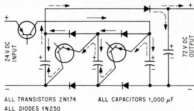
Three-stage d-c to d-c converter. Solid arrows show the charge cycle; dotted arrows show the discharge cycle.
