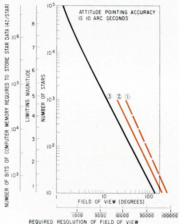
Design tradeoffs for three-axis attitude system. With wide field of view, the computer can operate with data on relatively few stars stored in its memory, and the detection system needs to consider only the brightest stars. However, this advantage requires high resolution in the field of view. Line 1 indicates conditions resulting in a 1.0 probability of finding three or more stars in field of view; line 2, probability of 0.9; line 3, an average of three stars.
