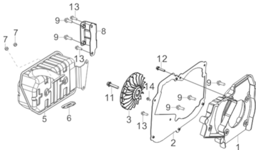
Fig. 11 - Muffler Assembly
