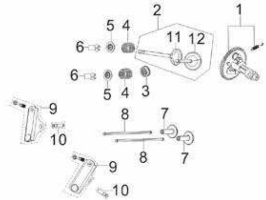
Fig. 6 - Valve Train & Camshaft Subassembly
