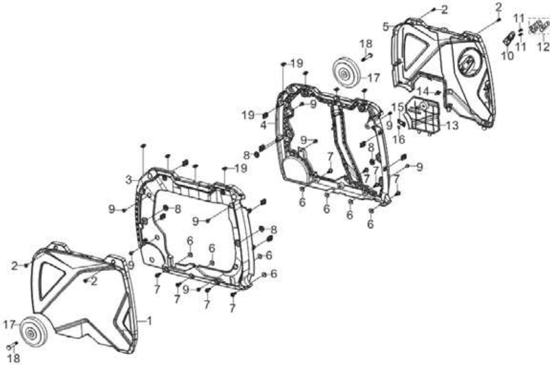
Fig. 16 - Side Covers
