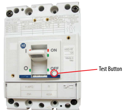
Position of the Contacts when the Circuit Breaker is TRIPPED via the TEST Button on the face of the Circuit Breaker or Shunt Trip or Undervoltage Release.
