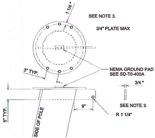
DETAIL "A" STATIC SUSPENSION OR DEADEND
