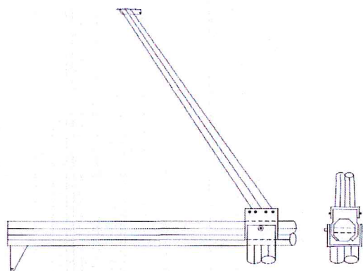
ARM CONNECTION DETAIL
