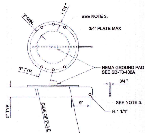
DETAIL "B" STATIC SUSPENSION OR DEADEND
