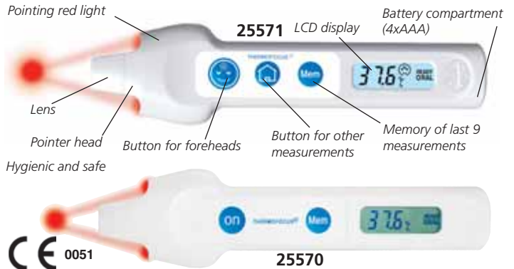
A patented optic-aiming system allows to immediately find correct distance for measurements.
