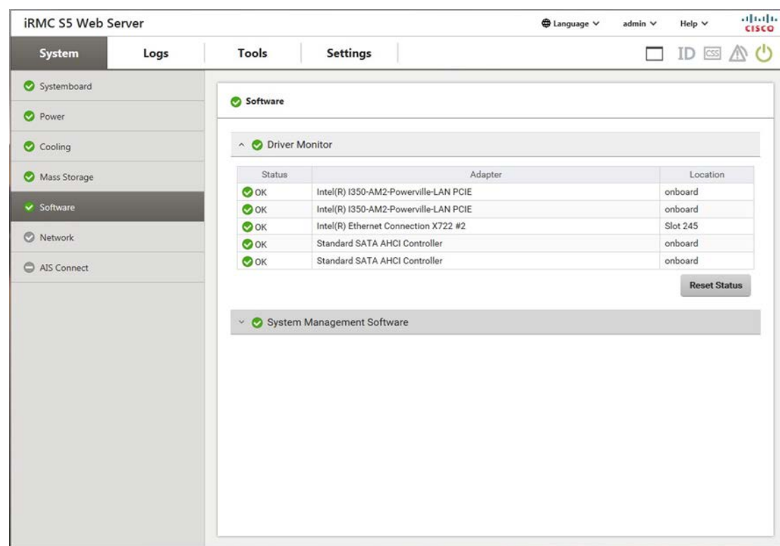
Figure 8: Software page
