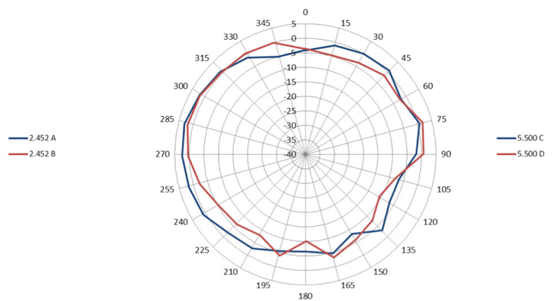
5.500GHz
