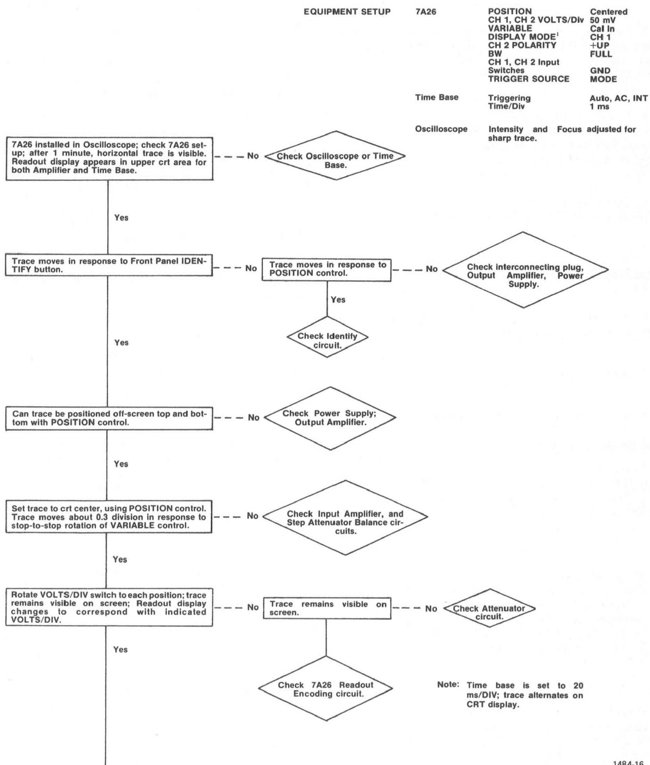
Fig. 4-1. Troubleshooting chart.
