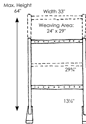
24" Tapestry Loom
