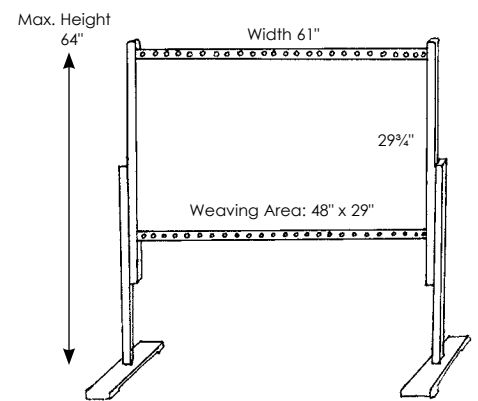
48" Tapestry Loom
