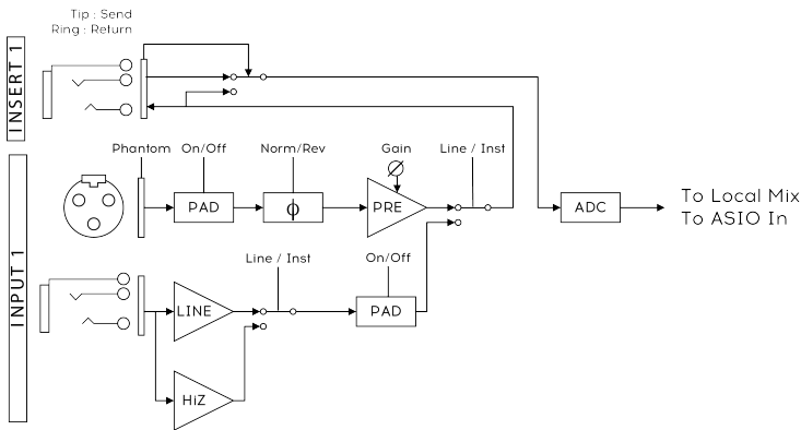
Input channel 1&2 path
