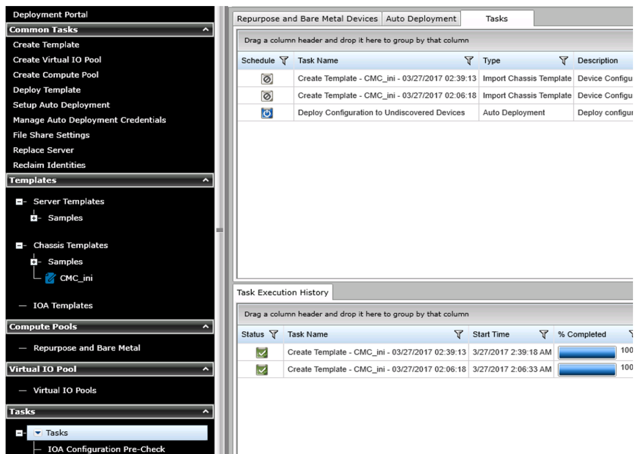
Figure 29 CMC Template Recreate Task
