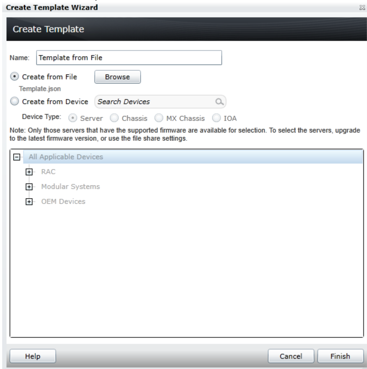
Figure 40 Create Template from a JSON File
