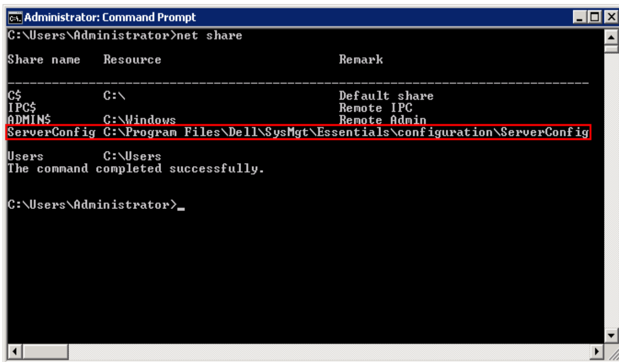
Figure 45 Net Share Command Results
