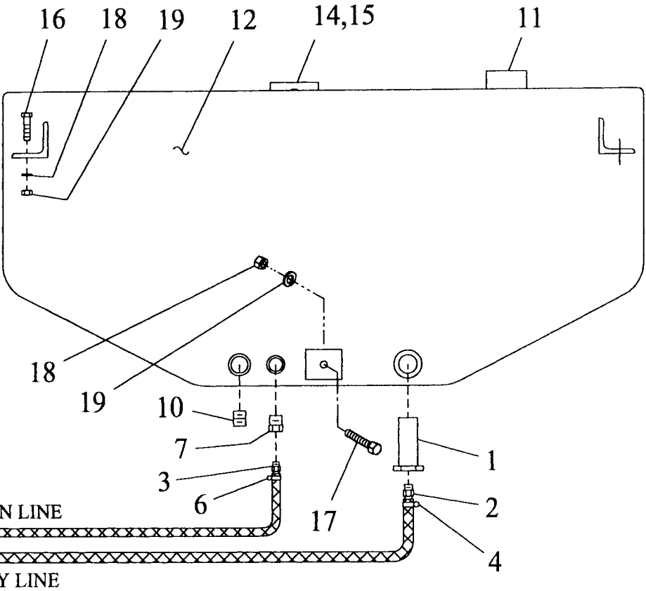
VIEW FROM RIGHT SIDE
