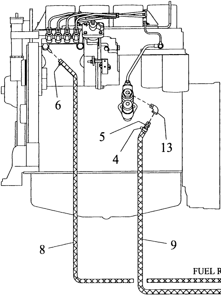
VIEW FROM LEFT SIDE
