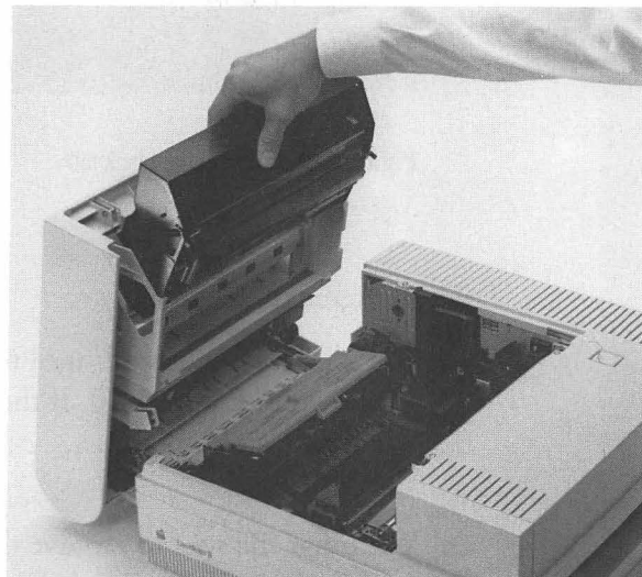
Figure 1-8 Inserting the toner cartridge
