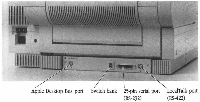
Figure F-1 The LaserWriter IINT connector panel
