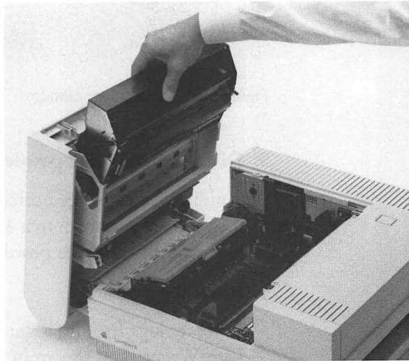
Figure 6-5 Removing the old toner cartridge
