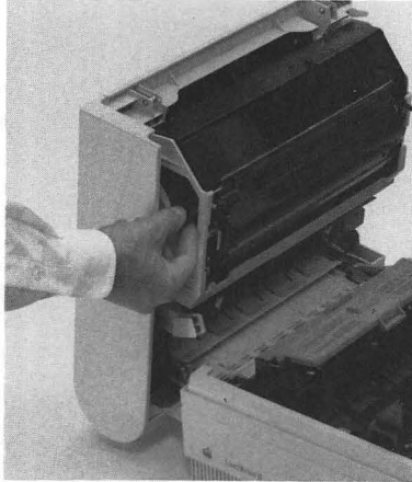
Figure 6-9 Flexing the black tab
