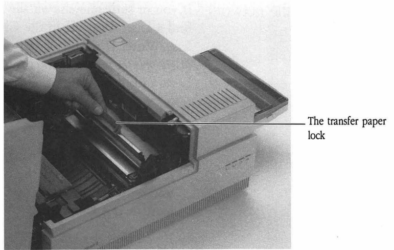
Figure 7-3 Opening the transfer paper lock
