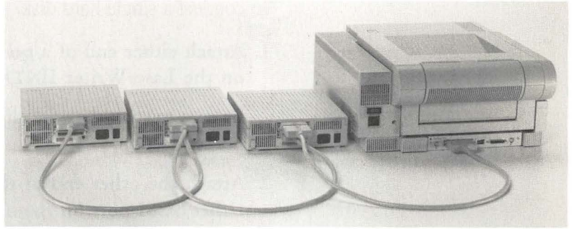
Figure B-2 Three hard disks connected to a LaserWriter IINTX
