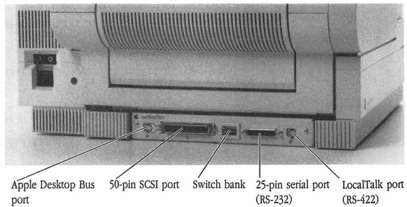
Figure F-2 The LaserWriter IINTX connector panel
