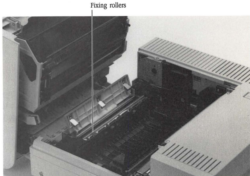
Figure 6-1 The fixing rollers
