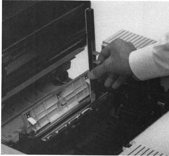
Figure 6-11 Cleaning the fixing rollers
