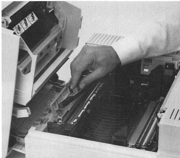
Figure 6-13 Installing the new cleaning pad
