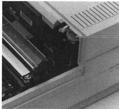
Figure 7-5 Adjusting the print density dial
