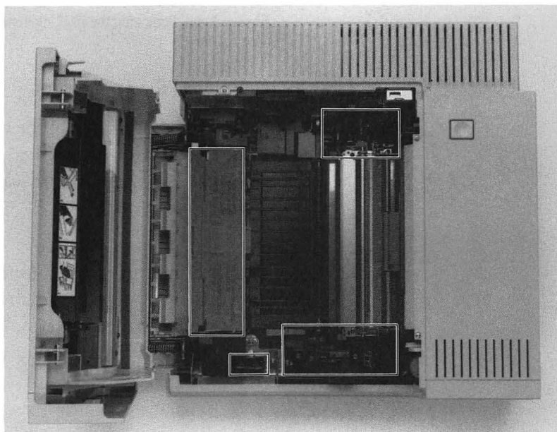
Figure 1-3 The interior of the LaserWriter II
