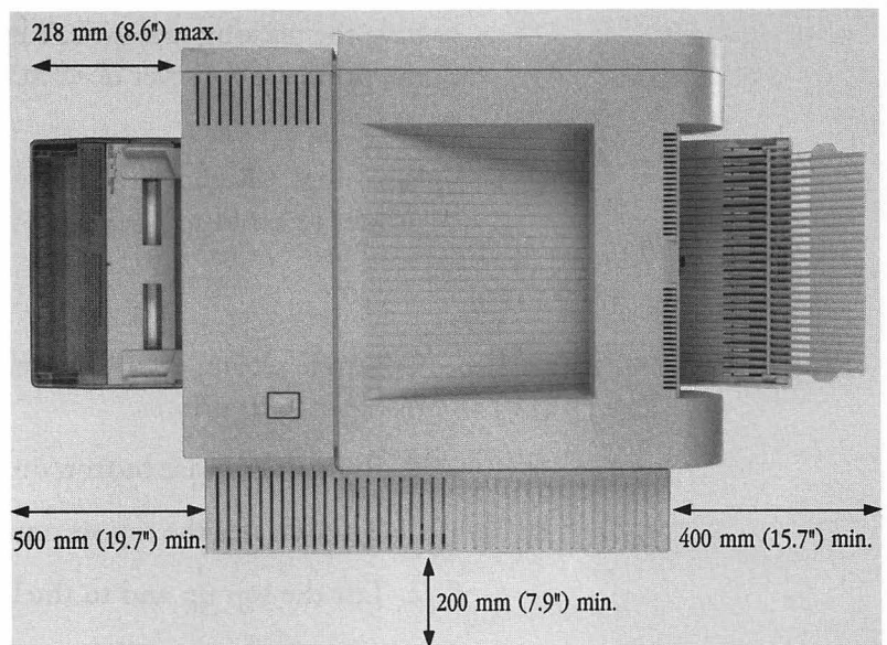
Figure 1-1 Dimensions of the LaserWriter II and the work area
