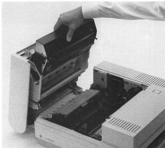
Figure 6-8 Inserting the toner cartridge
