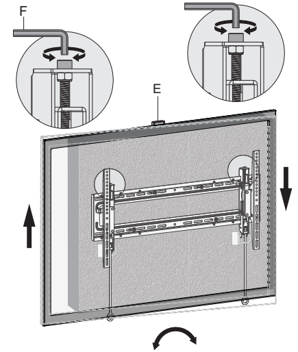
Level Adjustment
