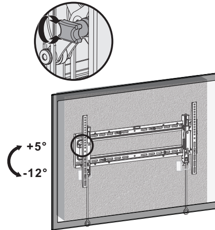
Tilt Adjustment
