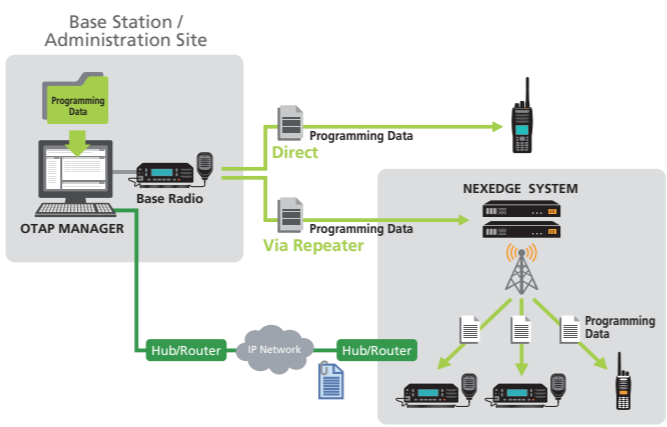
[ NEXEDGE OTAP (KPG-150AP/180AP) ]
