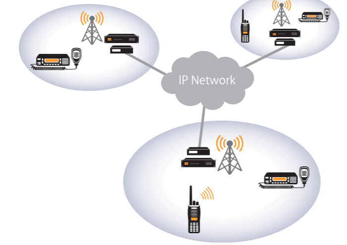
[ Conventional IP Network ]
