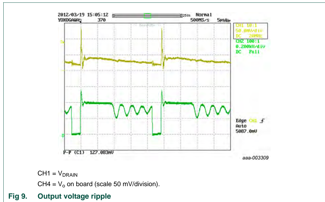
Figure 9 shows the output voltage ripple at a 1 A load at 230 V. The output ripple voltage is 127 mV using output capacitors C5 and C6 (820 \mu F/6.3 V Nichicon RL80J821MDN1KX).
