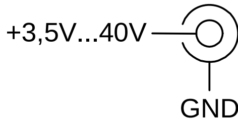
Figure 6-3 Power connector pinout (Roka 520 2550)
