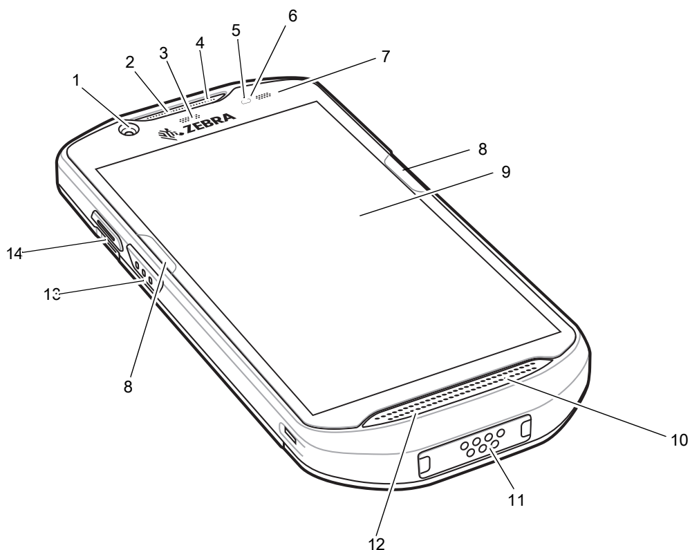
Figure 2 Front View
