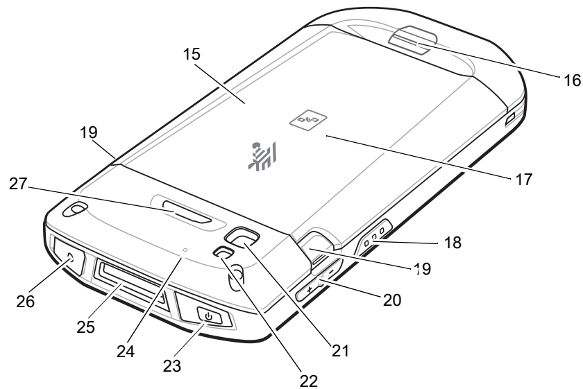
Figure 3 Rear View
