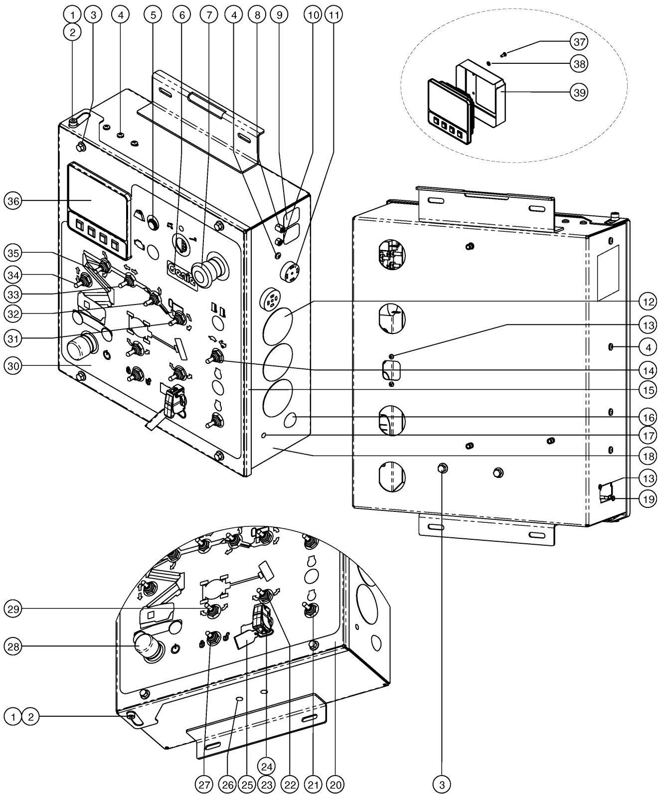
307.1 Ground Controls, with LCD Readout Screen, External View (For Deutz TD 2213)
