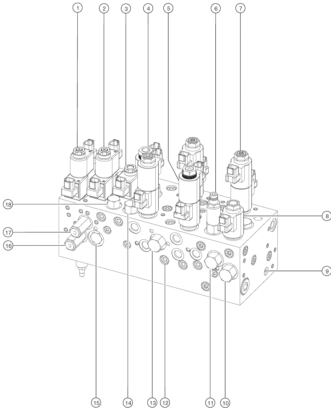
704.1 Function Manifold, View 1
