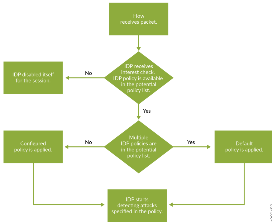
Figure 2: IDP Processing for Flow First Path
