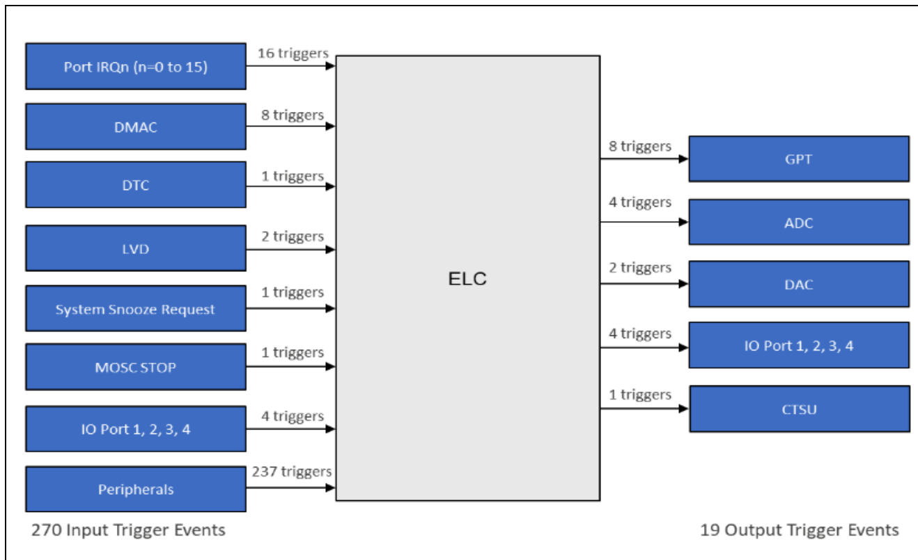
Figure 2 ELC Hardware Block Diagram
