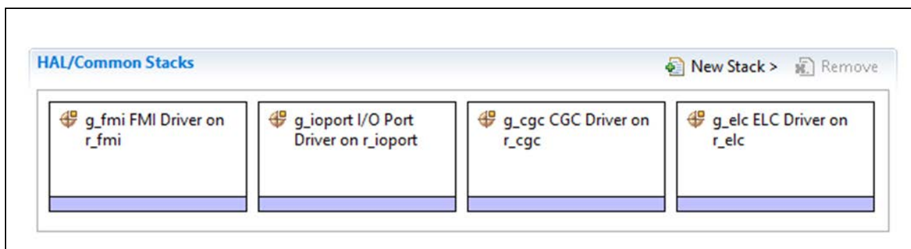
Figure 4 ELC HAL Module Stack
