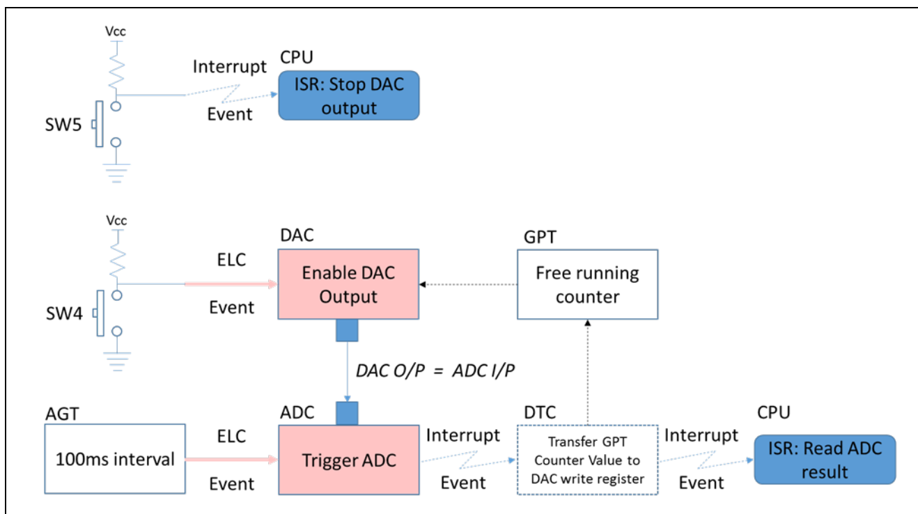
Figure 5 ELC HAL Module Application Project Architecture Diagram
