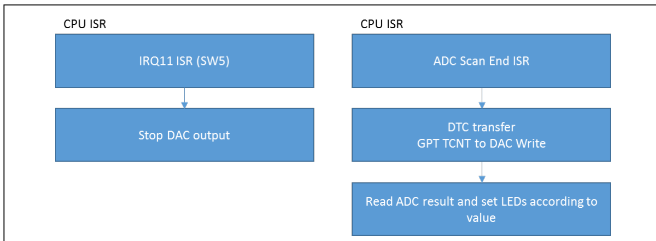
Figure 6 ELC HAL Module Application Project CPU ISR Diagrams
