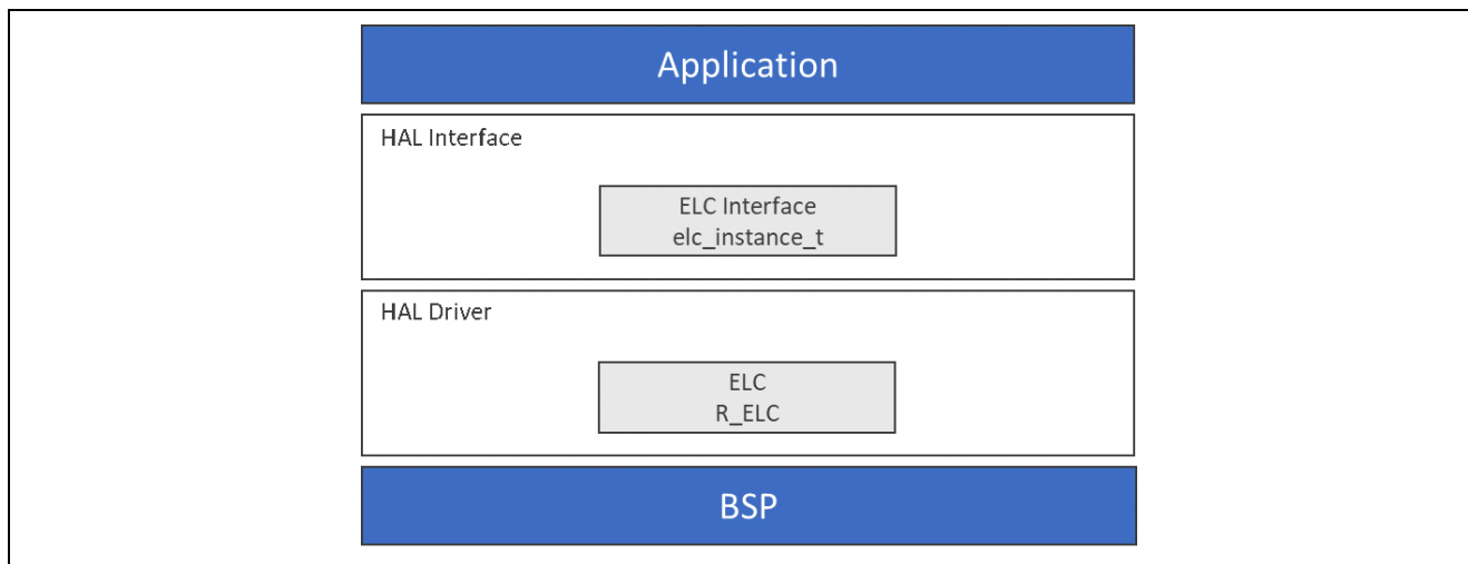
Figure 1 ELC HAL Module Block Diagram
