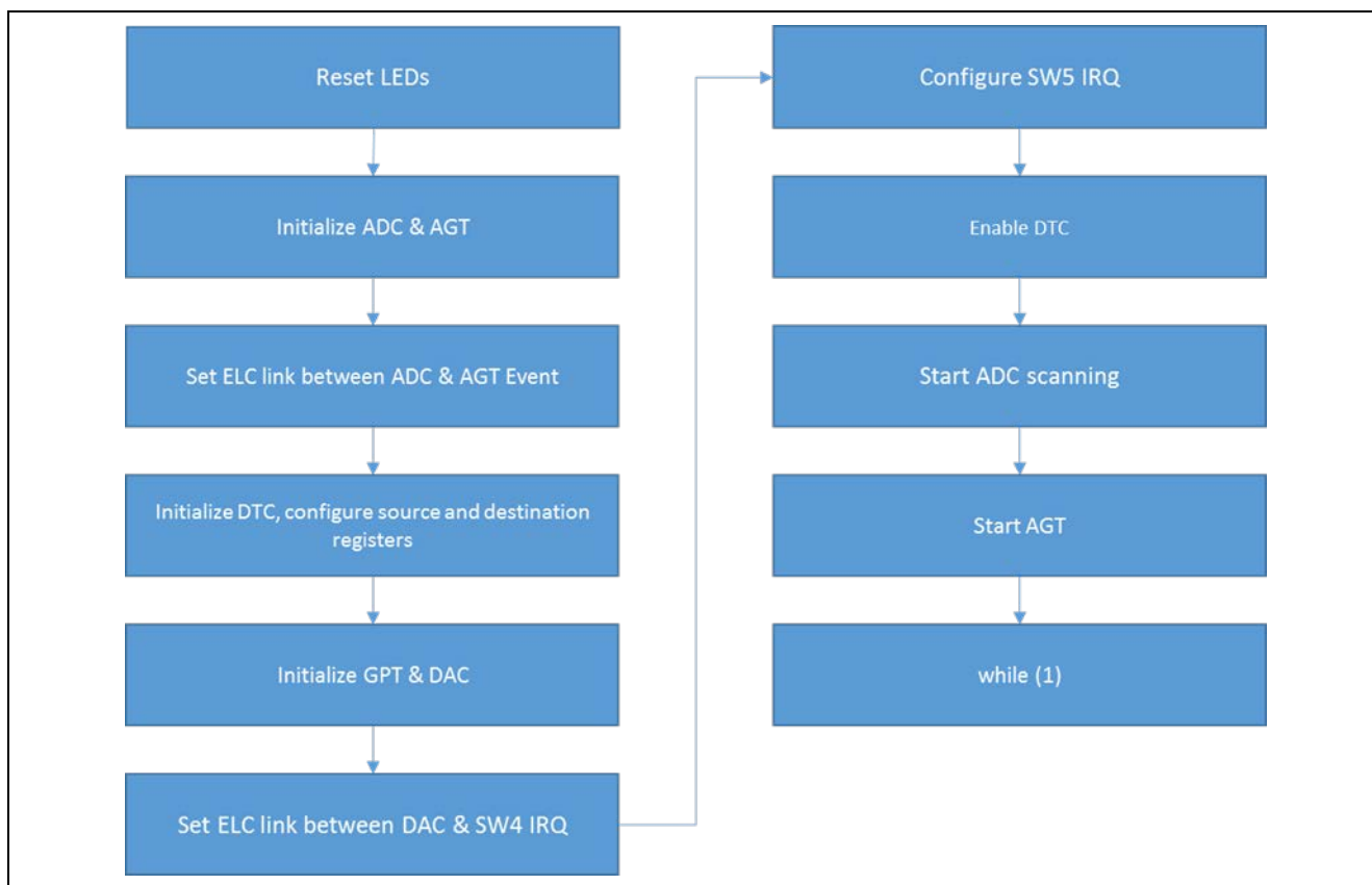
Figure 4 ELC HAL Module Application Project Flow Diagram
