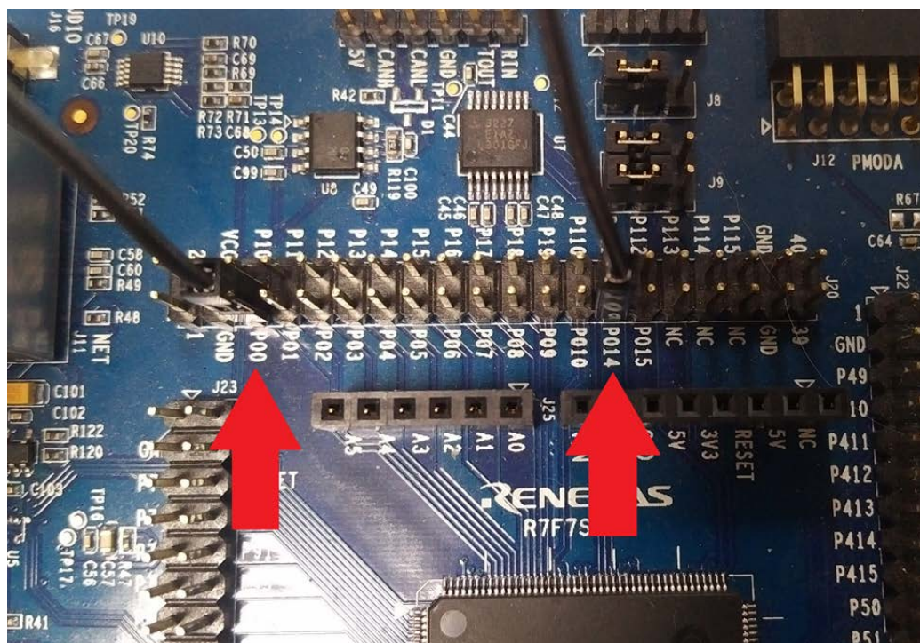
Figure 8 Connecting DAC output pin (P014) with ADC input pin (P00)
