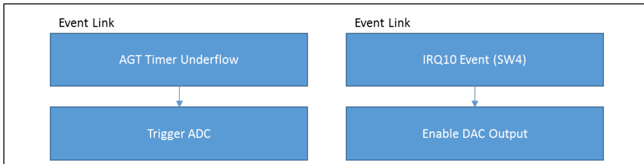
Figure 7 ELC HAL Module Application Project Event Link Diagrams
