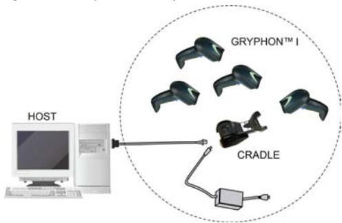
Figure 11. Multiple Reader Layout
