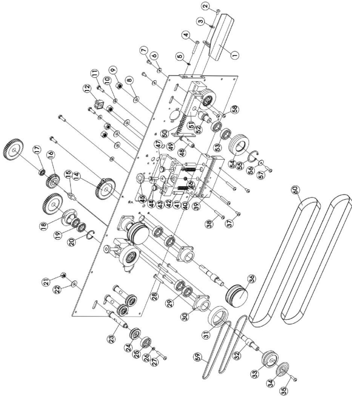
Figure 36. Spare Parts Diagram Overview
