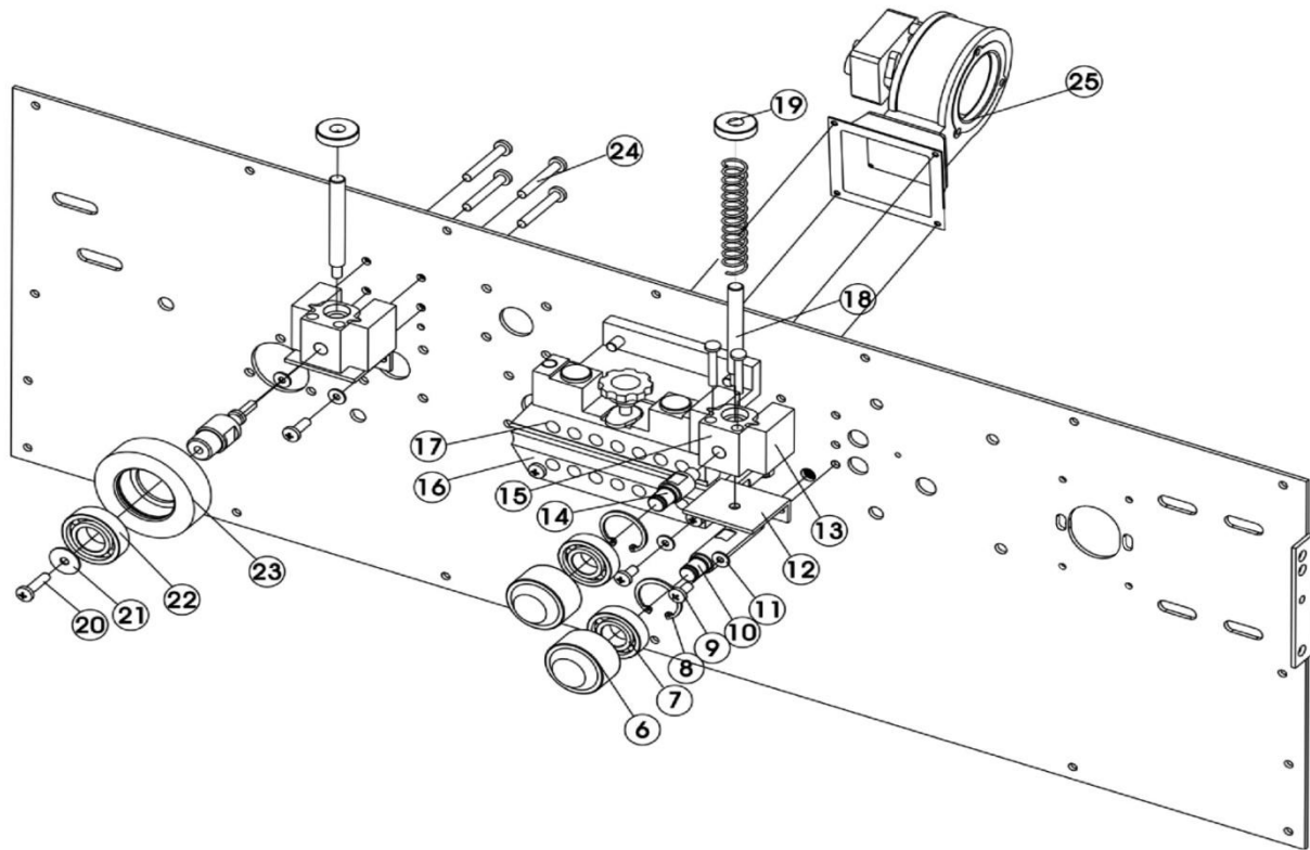
Figure 38. Heating / Cooling Blocks
