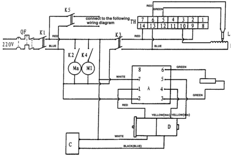
Figure 4. Electrical Circuit Diagram.
