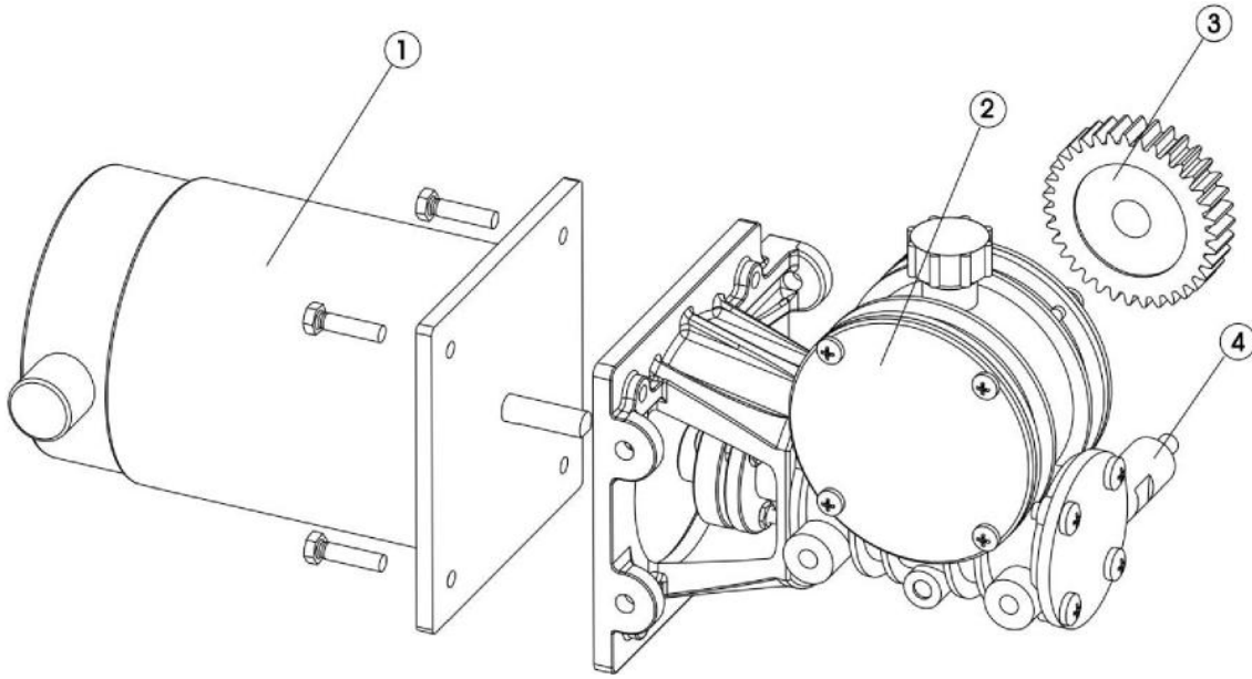
Figure 44. Motor / Turbocase
