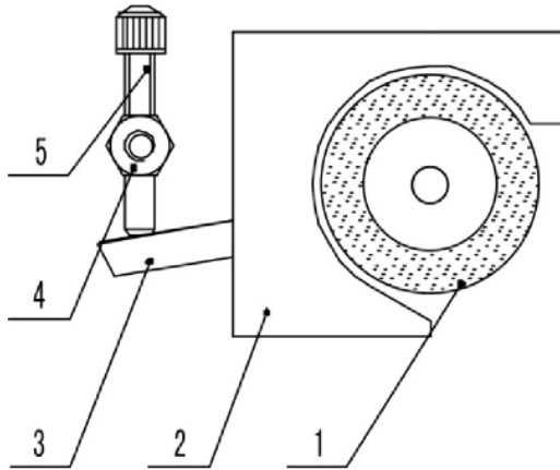
Figure 24. (1) Ink Roller, (2) Ink Roller Heating Block, (3) Swing Pole, (4) Adjusting Strut, (5) Ink Wheel Adjusting Device
