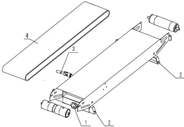
Figure 7. (1) Adjusting Knob, (2) Foot Rest, (3) Gimbal Assembly, (4) Conveyor Belt.
