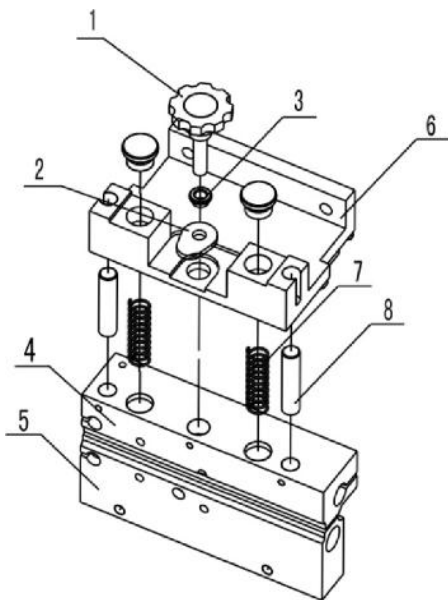
Figure 6. (1) Control Block Knob, (2) Adjusting Nut, (3) Nut, (4) Upper Heating Block, (5) Lower Heating Block, (6) Block Holding Plate, (7) Spring, (8) Guide Post
