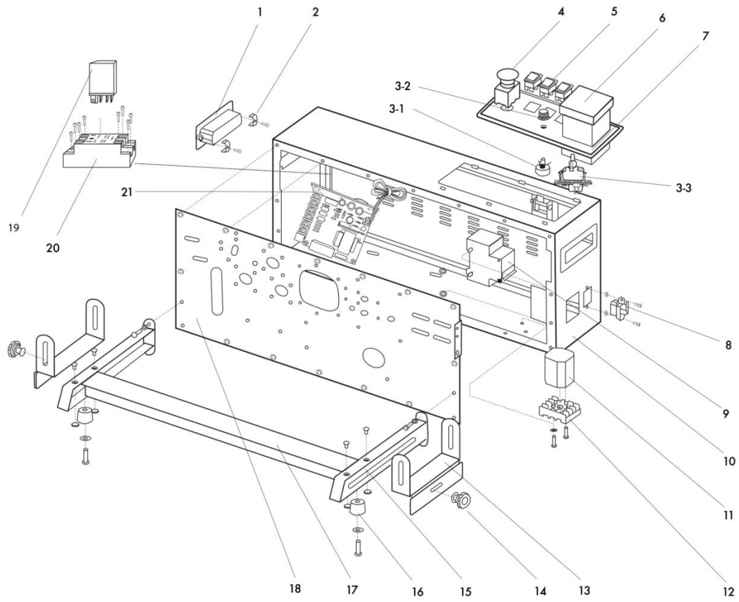
Figure 45. Sealer Body
