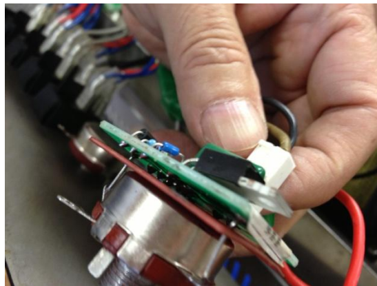
Figure 35. Unplug Ink Temperature Potentiometer w/ PC Board and Replace with a New Ink Temperature Potentiometer w/ PC Board
