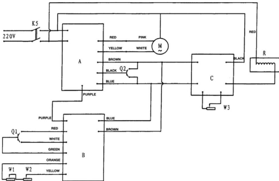
Figure 5. Electrical Circuit Diagram.
