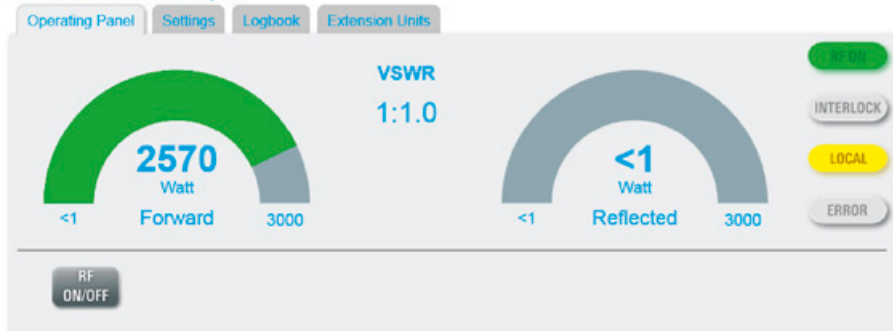
Operating panel on the R&S® BBL200 web GUI
