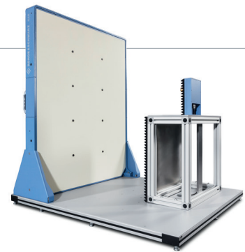
R&S®QAR Quality Automotive Radome Tester
