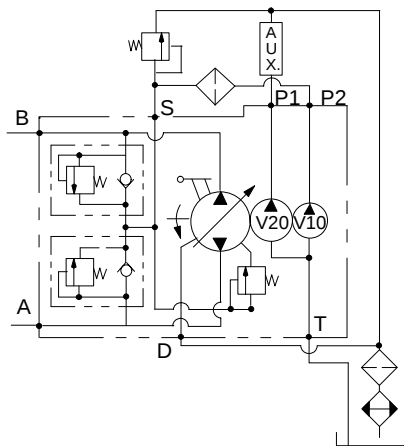
TA19V2010 with Main Relief Valves
