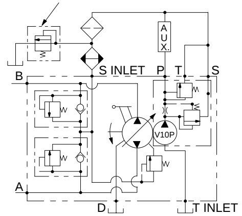
TA19V20P with Main Relief Valves
