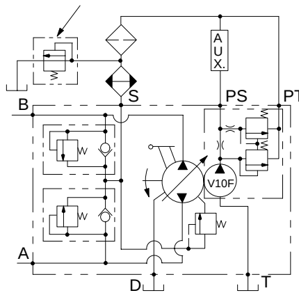
TA19V20F with Main Relief Valves
