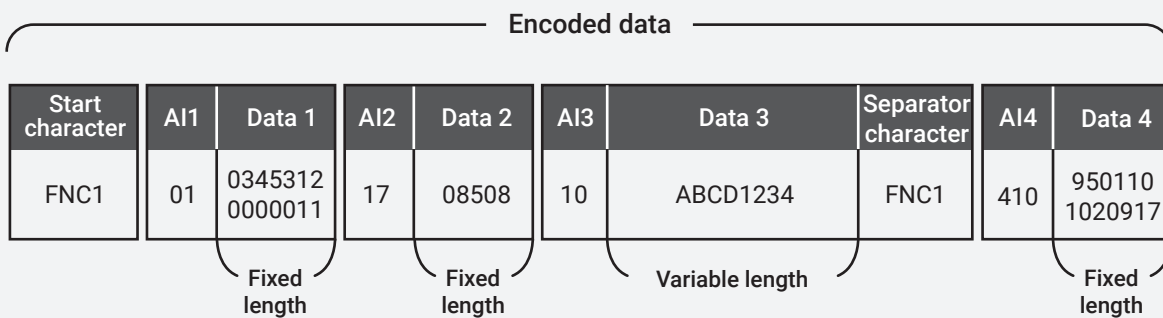
Structure of example code data
