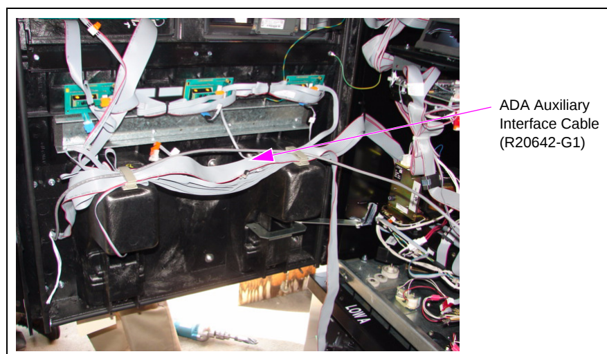
Figure 17: Clamping the ADA Auxiliary Interface Cable (R20642-G1)
