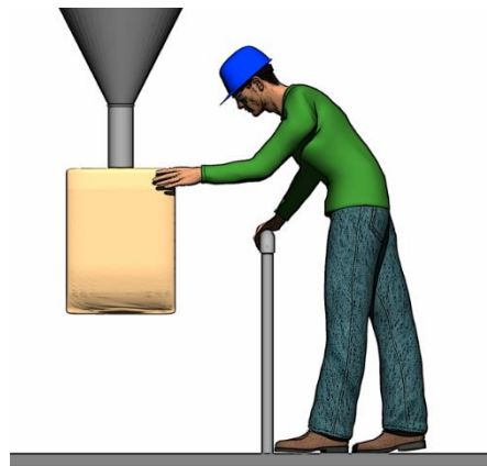
Figure 4. The guardrail is an obstruction. The worker must lean forward to place the bag on the spout. If the standing surface were closer to the spouts, the worker may not need to bend over as far and the guardrail could be modified to prevent the worker from falling onto the conveyor.
