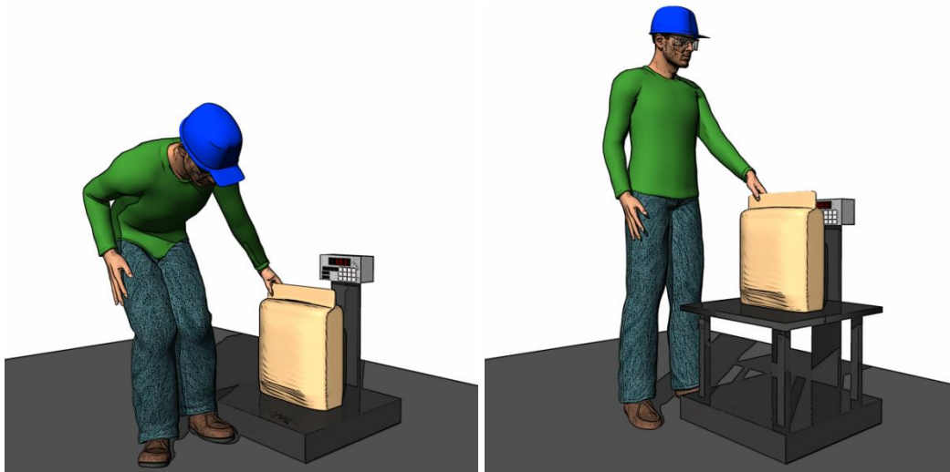
Figure 42. Scale placement on the ground requires worker to bend to pick up the bag from the scale (left). A table has been added on the scale to improve height and reduce bending required by workers (right).
