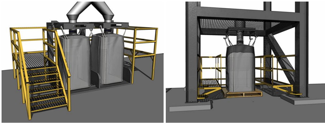
Figure 55. Platforms used to improve access to hooks and filling spout.
