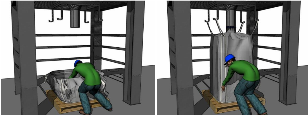
Figure 59. Worker is bending forward to reach inside and open the bag manually (left); worker is bending down to spread out the bottom corners of the bag during filling (right).
