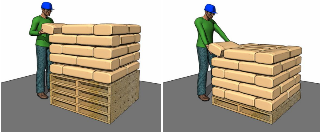
Figure 45. Method for using stacked pallets. Active pallet (fourth up from the ground on left) is placed on stack of inactive pallets and loaded until the top layer of bags is at 50 in from the ground (left), and pallet is moved by forklift to ground (right) and loading continues. Pallet on right should be loaded until the top layer of bags is 50 in from the ground.
