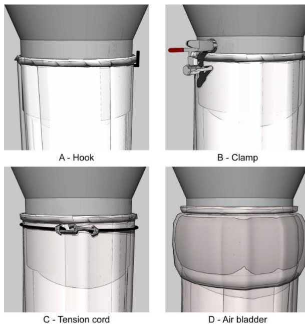
Figure 26. Methods of securing bag to filling spout.
