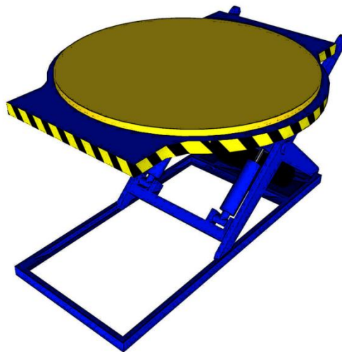
Figure 19. Turntable lift table. this style of table rotates and lowers as bags are placed on it.
