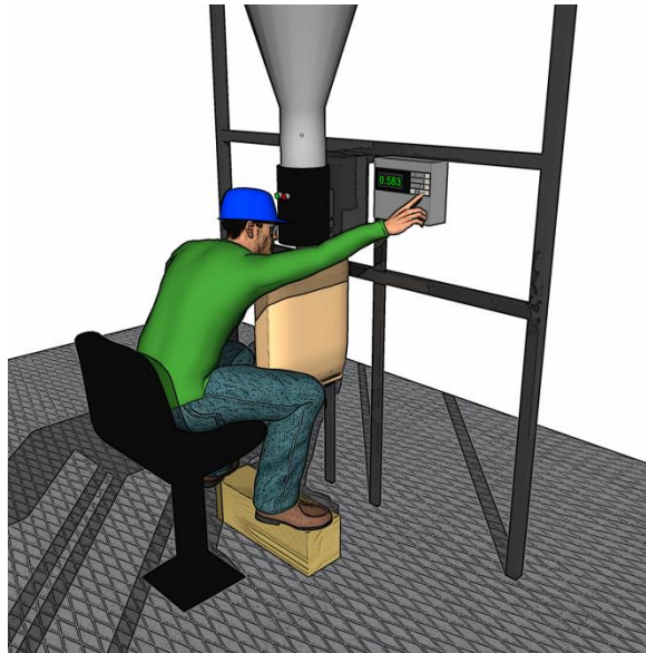
Figure 41. Location of controls requires worker to lean forward and reach with the arms, increasing injury risk for both the back and arms.
