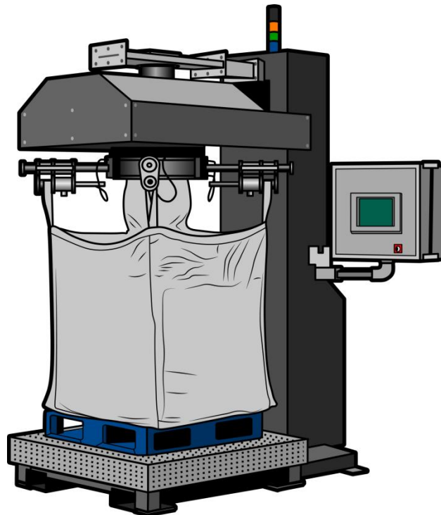
Figure 57. Example of filling station with rotating hooks.
