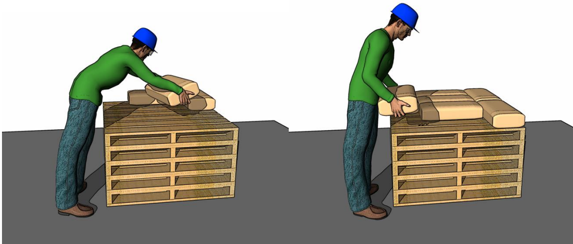
Figure 20. The pallet can be a barrier, requiring reaching away from the body to place the bag (left). The bag should be kept close to the body during all parts of the lifting/lowering process (right).
