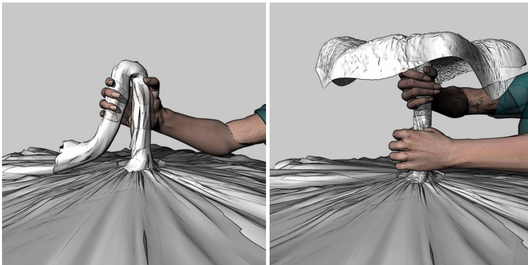
Figure 63. Snaking the liner of a bag (left) and flowering the liner (right)
