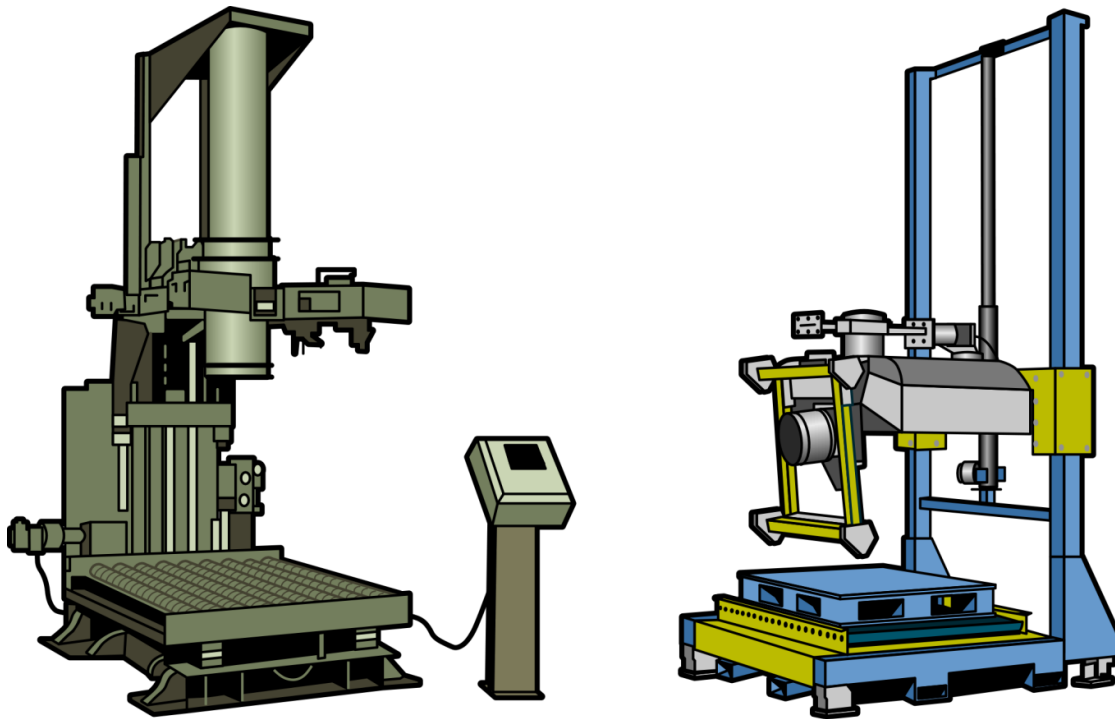
Figure 54. Examples of an adjustable height filling machine: National Bulk Equipment’s cantilevered models are standard with height adjustment (left), Flexicon’s SWING-DOWN® Bulk Bag Filler (right).
