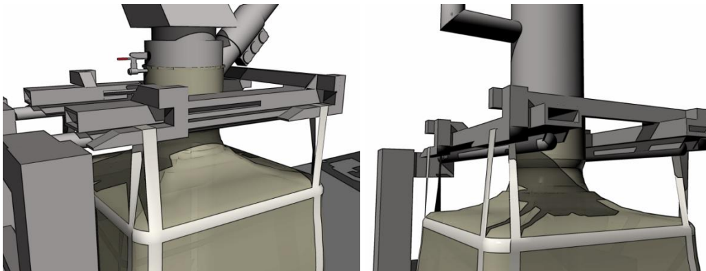
Figure 56. Bag filling stations with hooks mounted on frame that can be removed and lowered with a forklift.
