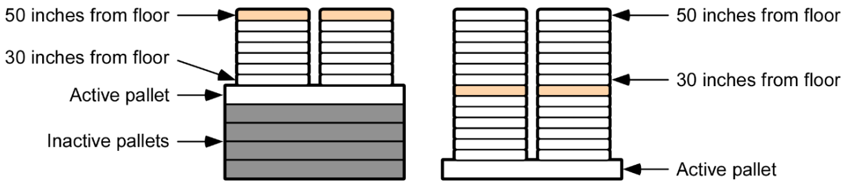
Figure 44. Method for using stacked pallets to improve postures during palletizing when a lift table is not possible. Step 1: Use 4 inactive pallets (shaded gray) to raise the height of the active pallet that is loaded so that the height of the first layer of bags is around 30 in. Load the active pallet until the top layer of bags is around 50 in (end of step 1 shown on left). Step 2: Use a forklift to move the active pallet from the top of the stack of inactive pallets to the ground and continue loading until midpoint of top layer of bags is around 50 in (end of step 2 shown on right; top bag at end of step 1 is shaded tan).
