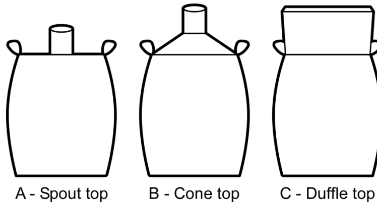
Figure 31. Types of bag tops.
