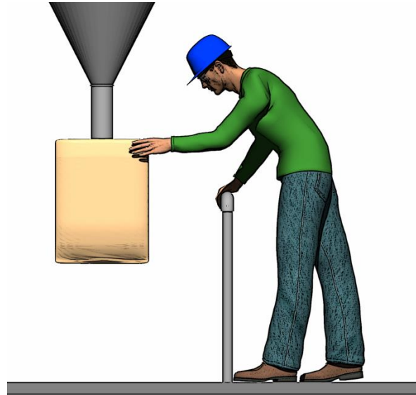
Figure 40. The guardrail is an obstruction. The worker must lean forward to place the bag on the spout. If the standing surface were closer to the spout, the worker may not need to bend over as far, and the guardrail could be modified to prevent the worker from falling onto the conveyor.
