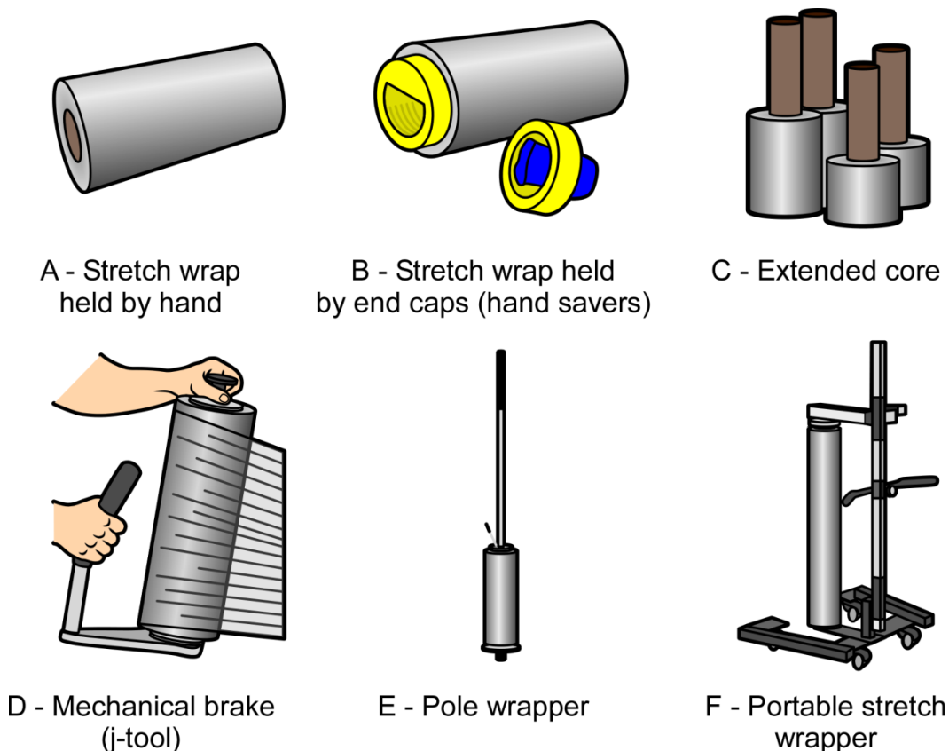
Figure 65. Tools used for stretch wrapping.
