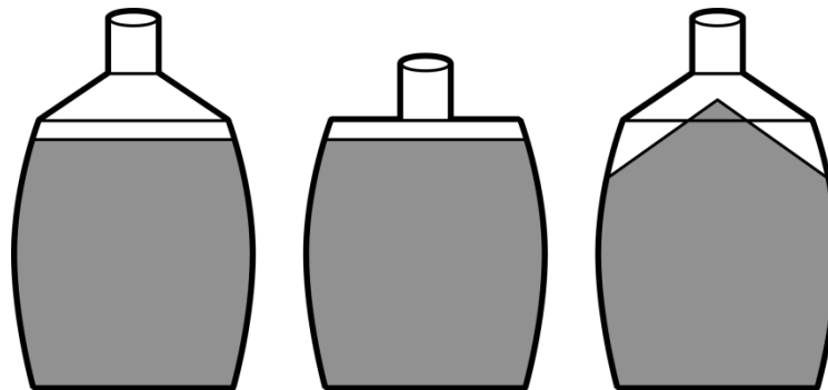
Figure 32. If the top of the product is flat during filling, the extra material at the top of the cone top bag is not filled and is unnecessary (left); product properly fills spout-top bag (center). A cone-top bag is only needed if the product piles in the center during filling (also referred to as having a high angle of repose, right).
