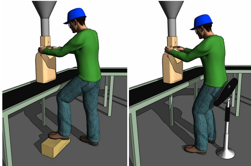
Figure 33. Possible solutions to prolonged standing postures: foot rest (left) and lean stand (right).
