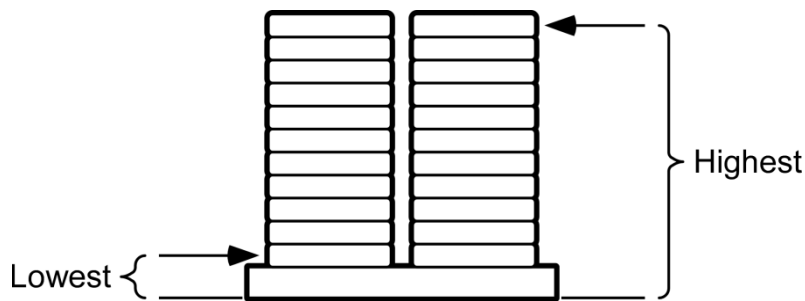
Figure 12. Lowest and highest bag measurement guidelines: Measure from the surface the worker is standing on to the center of the bag after it is placed on the pallet. Ensure that measurements of the bags are taken at the height they are loaded (e.g., if a lift table is used, the measurements of the bags are taken at the height they are loaded (e.g., if a lift table is used, the lowest and highest height may be the same).
