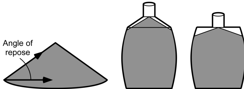
Figure 61. The angle of repose refers to the angle between a horizontal line and the surface of product (also referred to as the natural slope; left). A product with a high angle of repose will evenly fill a cone-top bag (center), but will leave unused space at the top corners of a spout-top bag and will require adjusting to evenly fill the bag (right).
