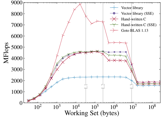
Figure 5: Single-threaded performance of double-precision dot product implementations. C implementations were compiled using GCC 4.8.1 and compiler options -O3 -msse4.2 -ffast-math -ftree-vectorize -funroll-loops . Sizes of the L1, L2, and L3 caches are marked.
