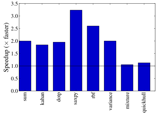
Figure 8: Speedup of benchmarks from using modified vector.
