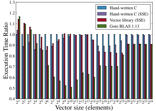
Figure 6: Relative performance of single-threaded ddot implementations. All times are normalized relative to the hand-written, compiler-vectorized, C implementation.
