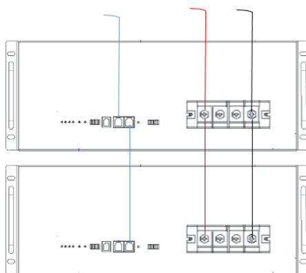
Pic. 8-2 48200 installation drawing
