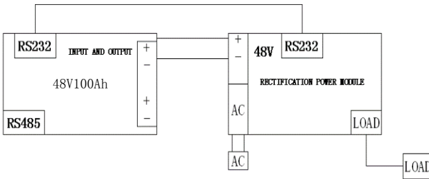
Pic. 7-1Working principle diagram of LFP battery module
