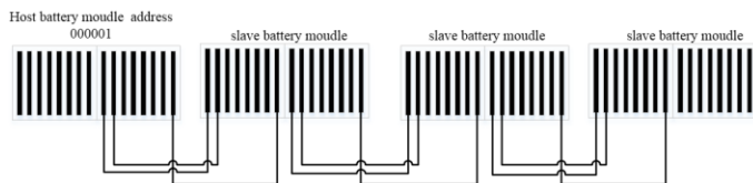
Pic. 6-2 The cascade communication wire connections of RS485
