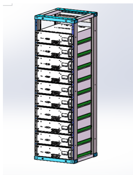
Pic. 8-4 ( n \times 100 ) Ah Communication LFP battery system ( n is the quantity of 48V100Ah battery modules )
