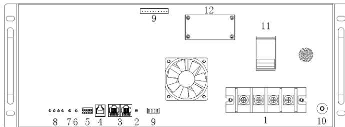
Pic. 6-1 Schematic drawing of the module panel
