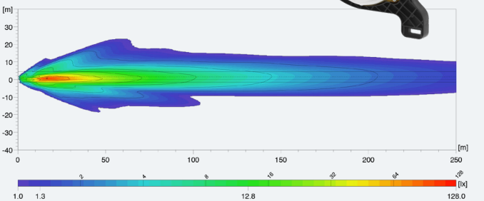
M133 Halogen (R149 Class B) (997 262)
