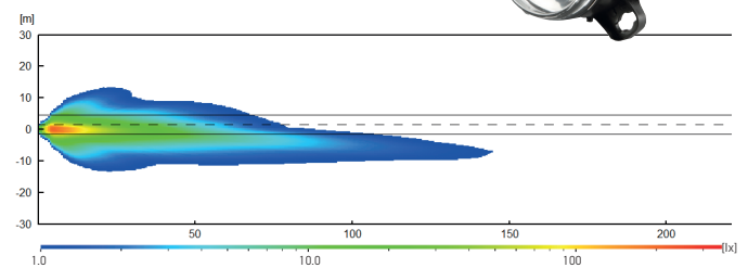
Halogen Performance (247 042)
