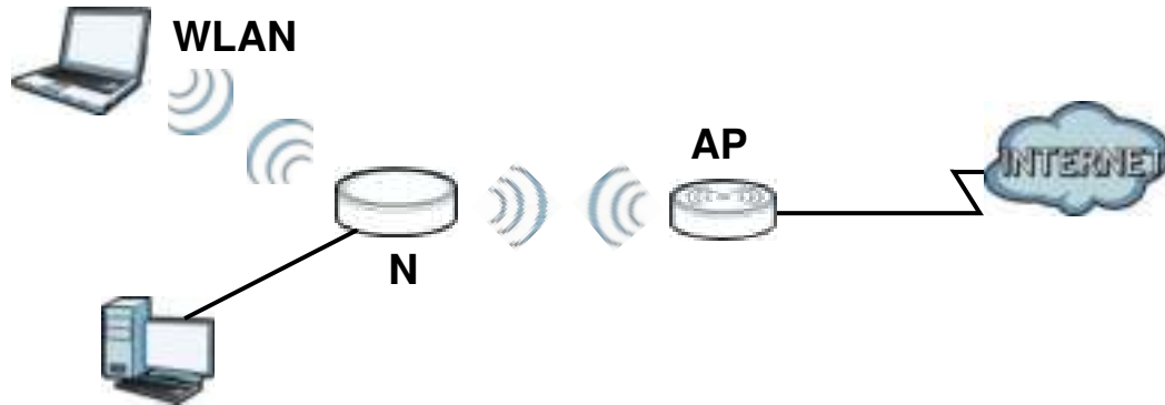
Figure 19 Universal Repeater
