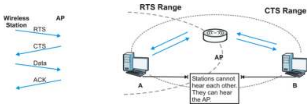
Figure 146 RTS/CTS
