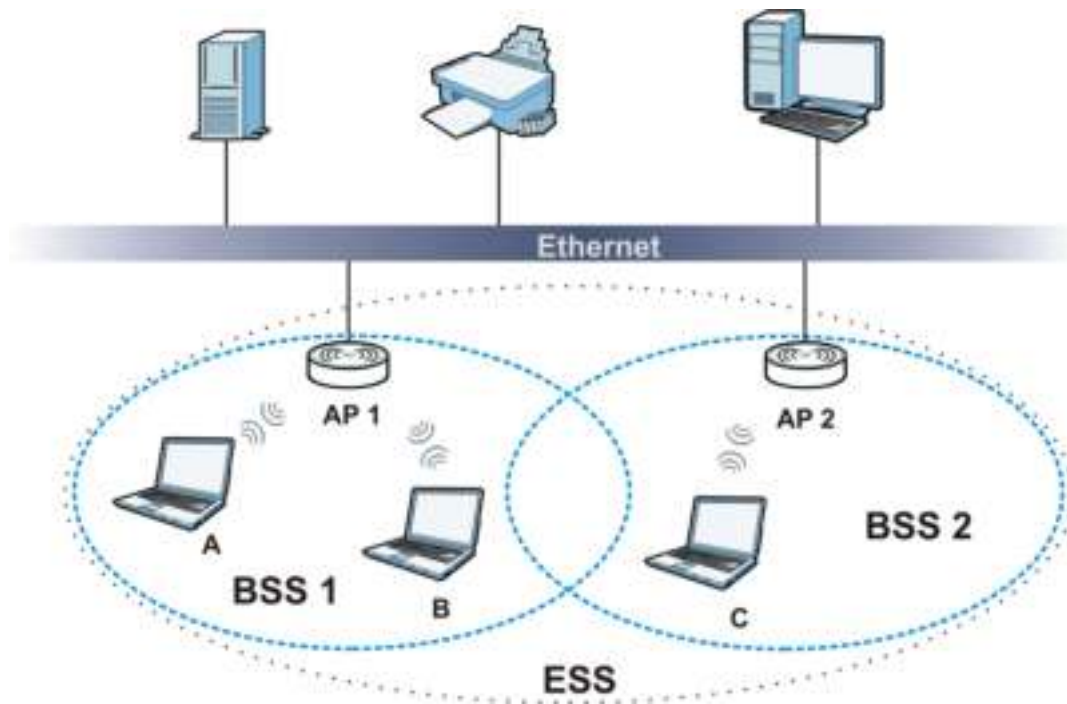
Figure 145 Infrastructure WLAN
