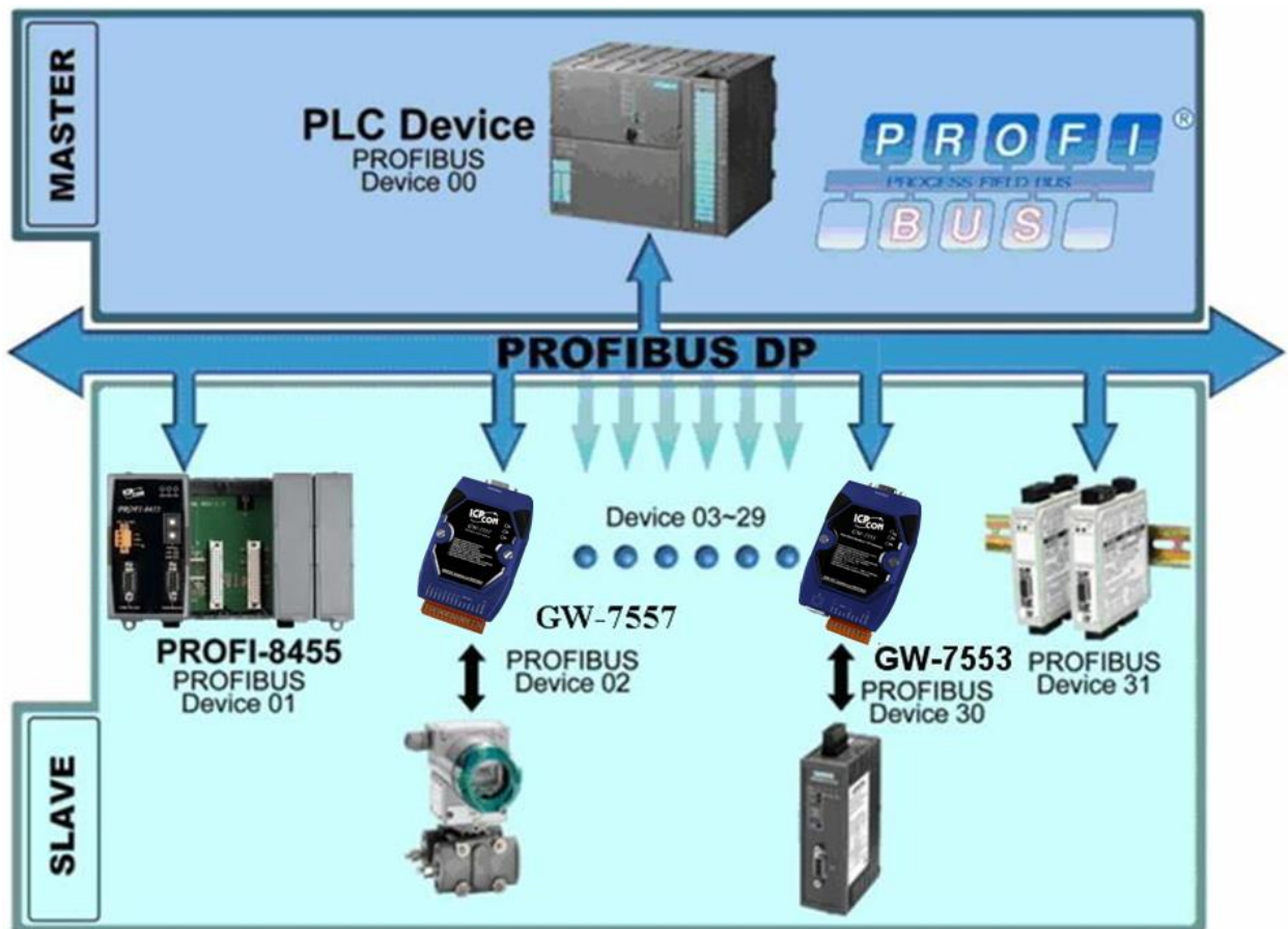
Figure 20 Mono-master system
