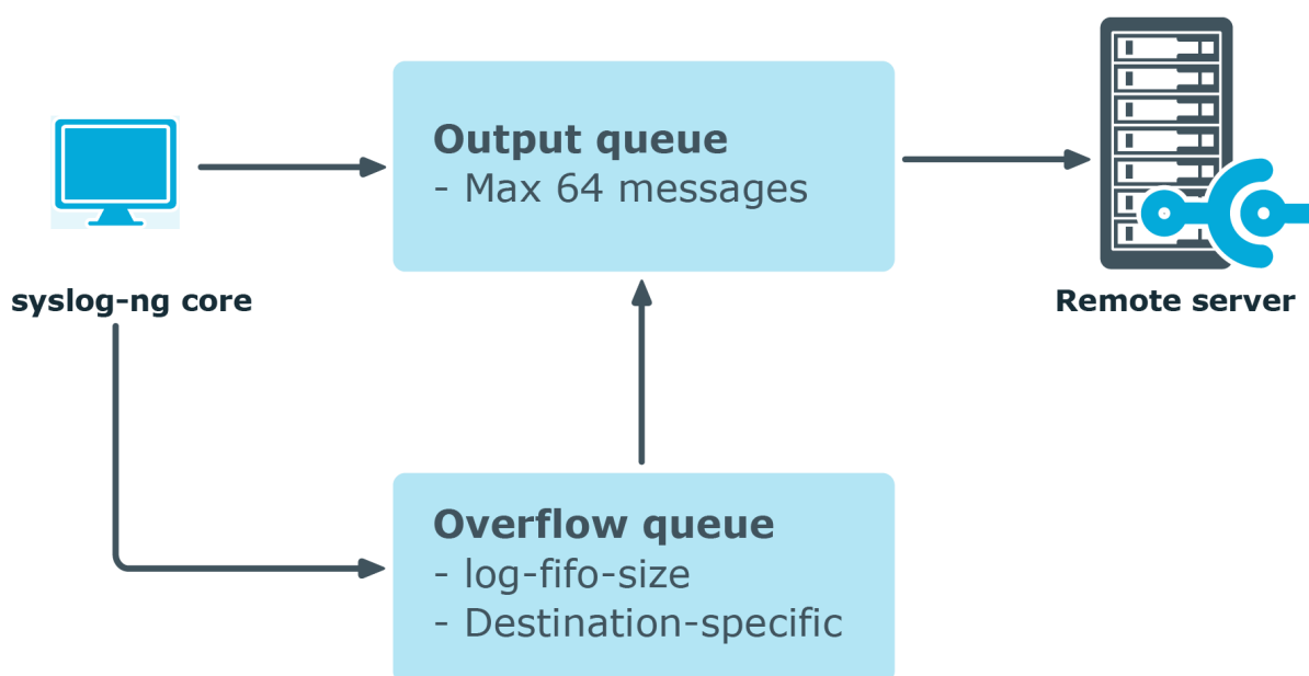
Figure 31: Handling outgoing messages in syslog-ng PE
