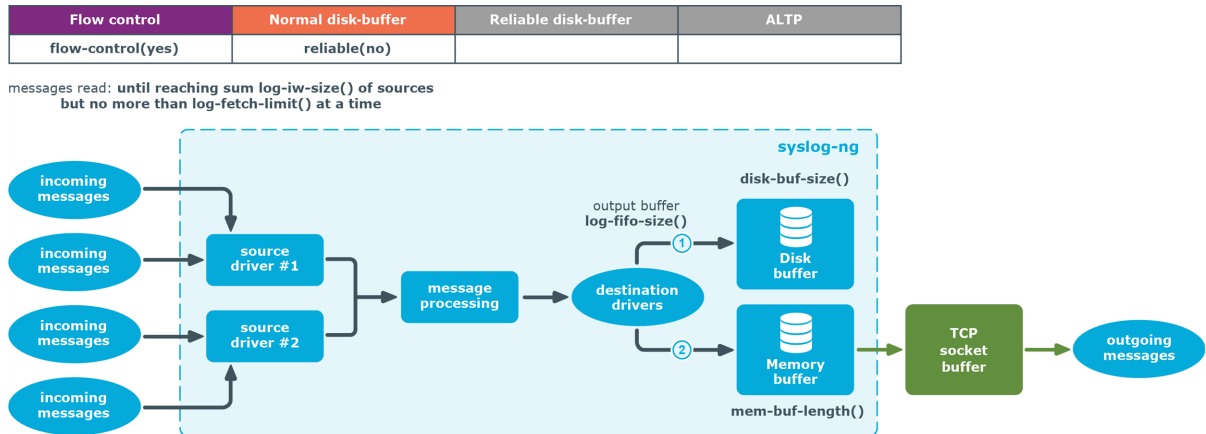
Figure 34: Flow control, normal disk buffering, no ALTP
