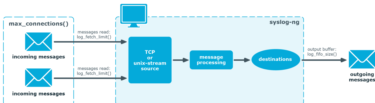
Figure 29: Managing log messages of TCP sources in syslog-ng PE
