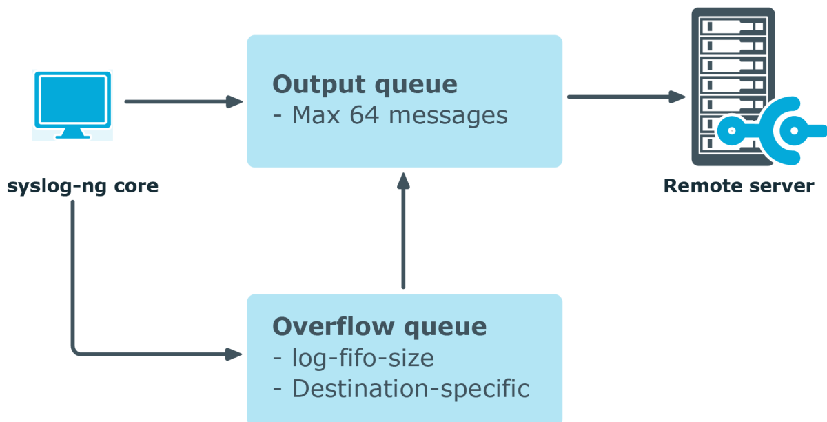
Figure 30: Handling outgoing messages in syslog-ng PE
