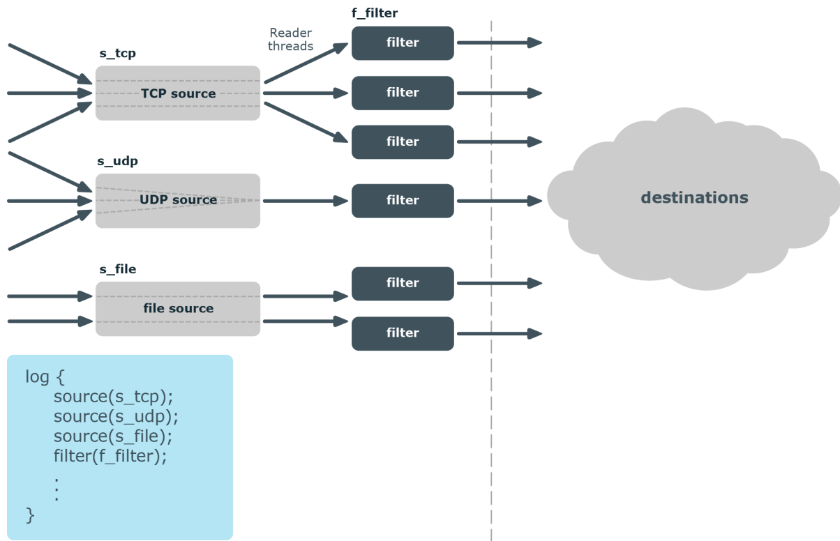
Figure 39: How multithreading works — sources
