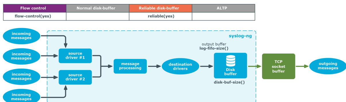
Figure 35: Flow control, reliable disk-buffer, no ALTP
