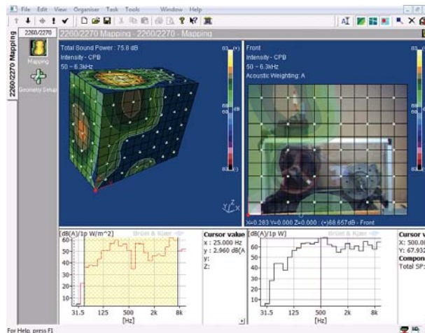
Fig. 5.11 A 3D contour map made using Type 7752 mapping software
