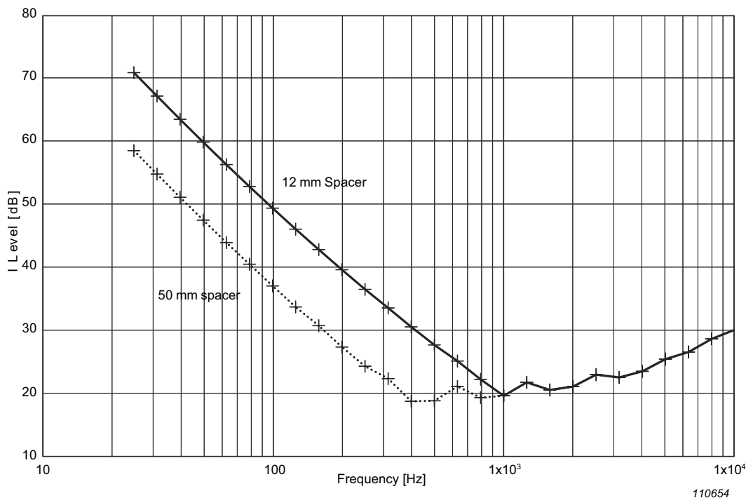
Fig. 6.12 The lower limit of the dynamic range for sound intensity measurements under all assumptions defined above
