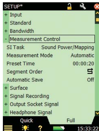
Fig. 3.17 Measurement Control setup
