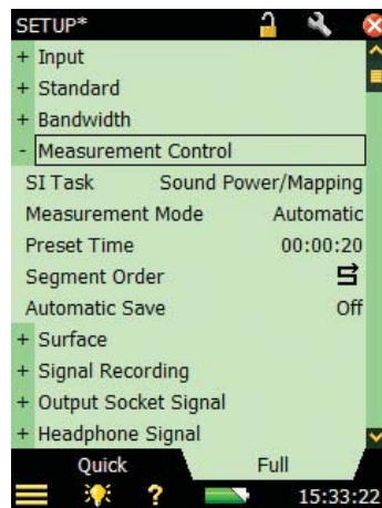
Fig. 3.34 Measurement Control setup
