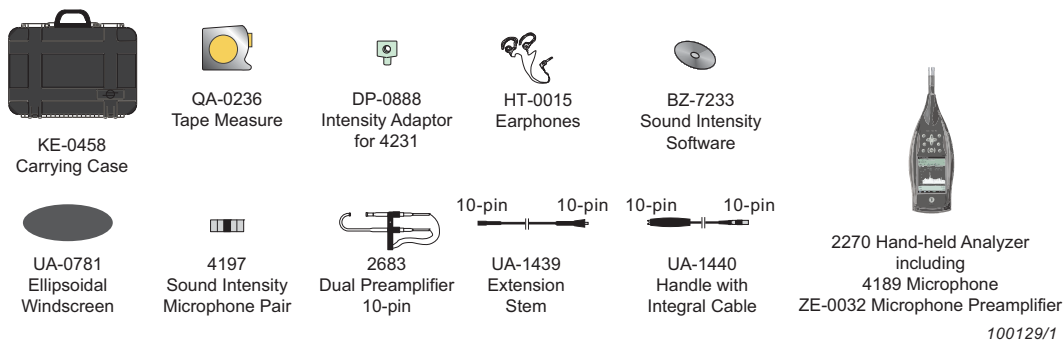
Fig. 2.2 System components for sound intensity measurements
