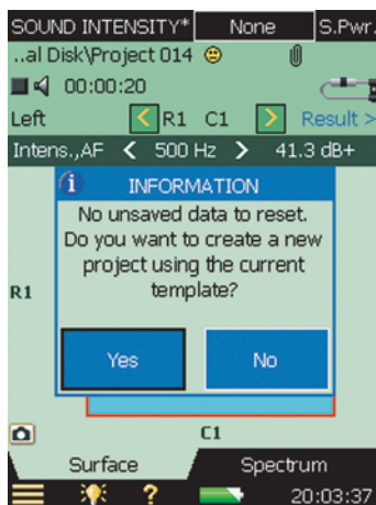
Fig. 5.10 Information pop-up
