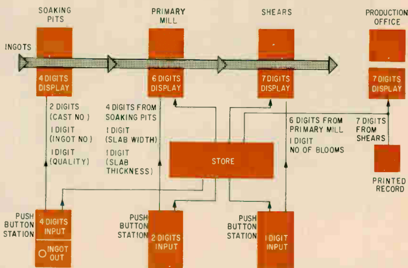
ROLLING MILL RUNNING RECORD —As work proceeds down the processing line its progress is signaled to the next station, and the production office winds up with a printed record (British Iron & Steel Research)
