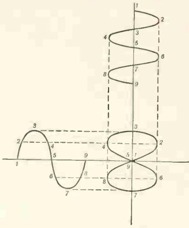
Construction of Lissajous figure.
