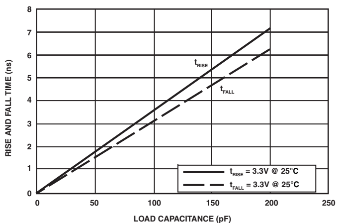
Figure 66. Driver Type D Typical Rise and Fall Times (10%–90%) vs. Load Capacitance ( 3.3V V_{DDEXT}/V_{DDMEM} )
