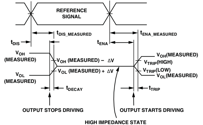
Figure 53. Output Enable/Disable
