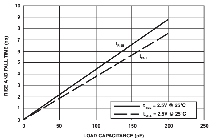
Figure 65. Driver Type D Typical Rise and Fall Times (10%–90%) vs. Load Capacitance ( 2.5V V_{DDEXT}/V_{DDMEM} )
