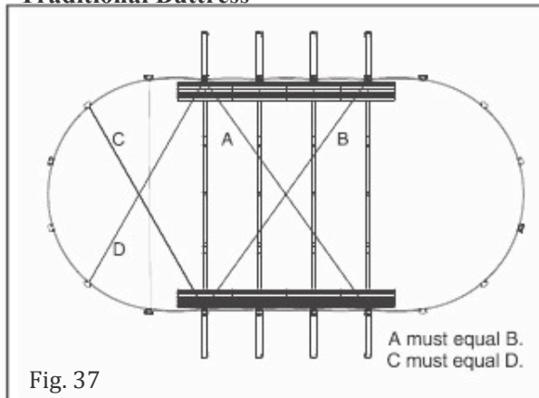
Traditional Buttress
