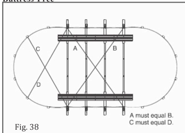
Buttress-Free
