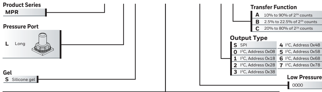
FIGURE 1. PRODUCT NOMENCLATURE FOR APPLICATIONS ABOVE 250,000 UNITS PER YEAR
