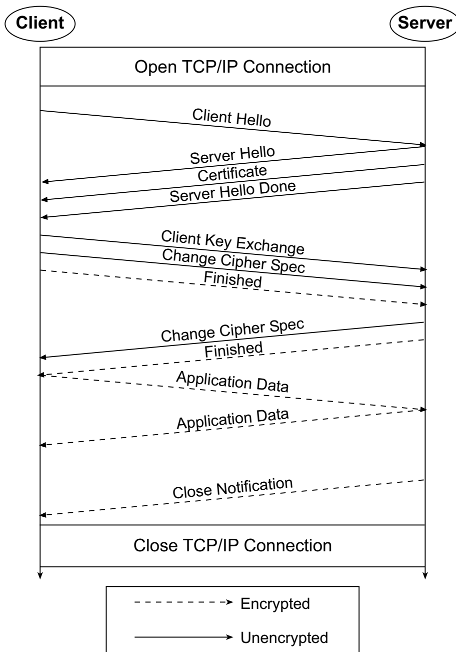
Figure 9. SSL Handshake
