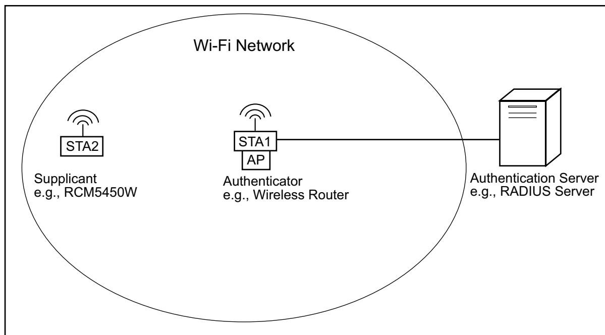
Figure 16. 802.1X Overview
