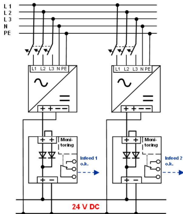
Figure 4: Configuration with one redundancy module for each power supply: SITOP PSE202U 24 V/ 10 A with one power supply unit up to 10 A or PSE200U 24 V/ 40 A with one power supply unit with a maximum of 40 A rated output current. Each of the two 24 V inputs on the redundancy modules is bridged
