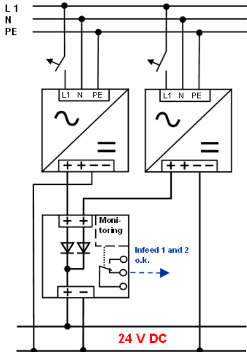
Figure 3: Configuration with one redundancy module for two power supplies: SITOP PSE202U 24 V/ 10 A with two power supply units up to 5 A or 24 V/ 40 A with two power supply units up to 20 A rated output current
