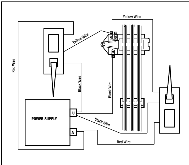
Figure 2. Accessory connection
