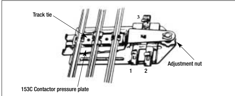
Figure 1. 153C Contactor
