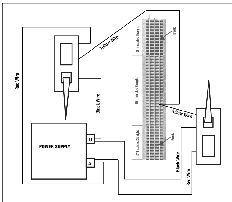
Figure 3. FasTrack connections
