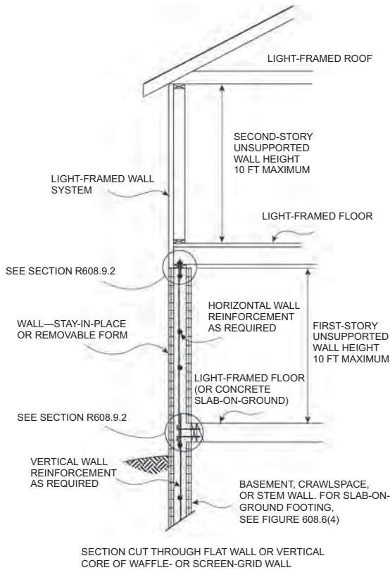
FIGURE R608.6(3) ABOVE-GRADE CONCRETE WALL CONSTRUCTION CONCRETE FIRST STORY AND LIGHT-FRAMED SECOND STORY
