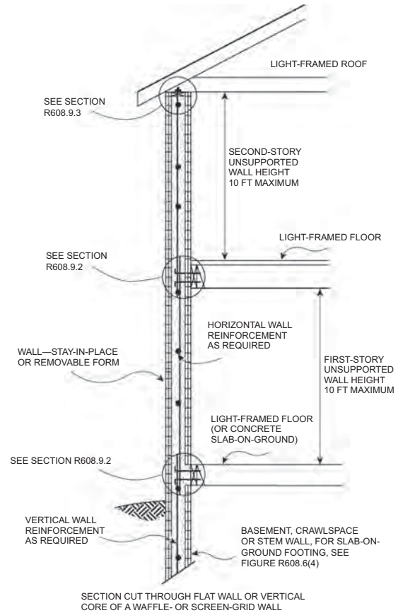
FIGURE R608.6(2) ABOVE-GRADE CONCRETE WALL CONSTRUCTION TWO-STOREY
