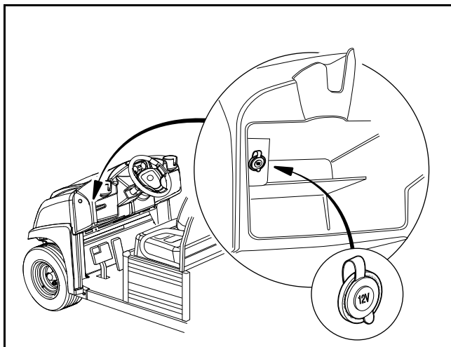
Figure 7 12-Volt Power Point
