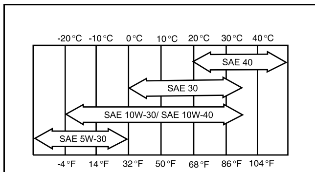
Figure 20 Oil Viscosity Chart
