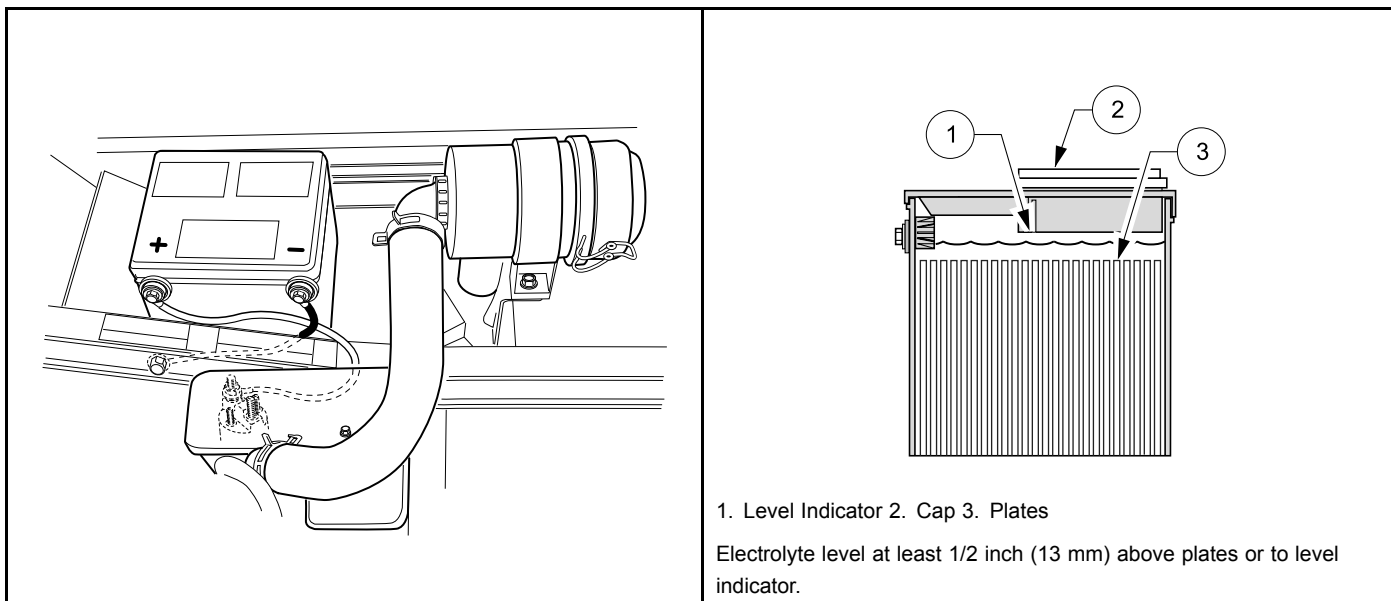
Figure 16 Gasoline Vehicle Battery
