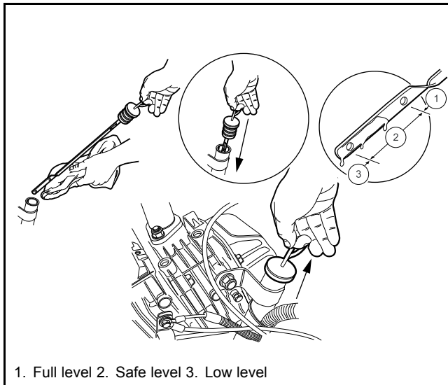
Figure 18 Engine Oil Level Check
