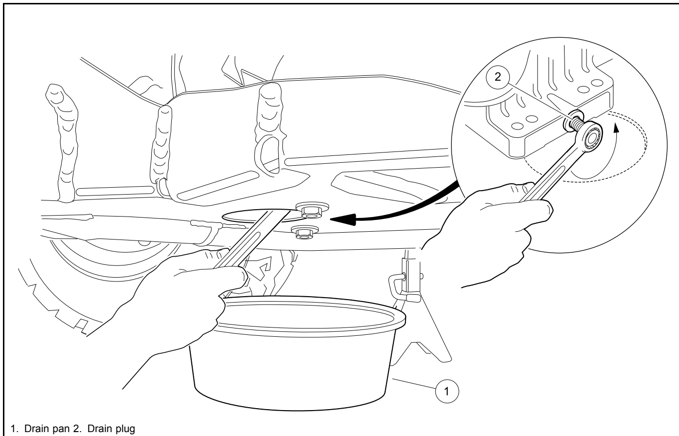
2667 Figure 19 Engine Oil Drain Plug and Pan
