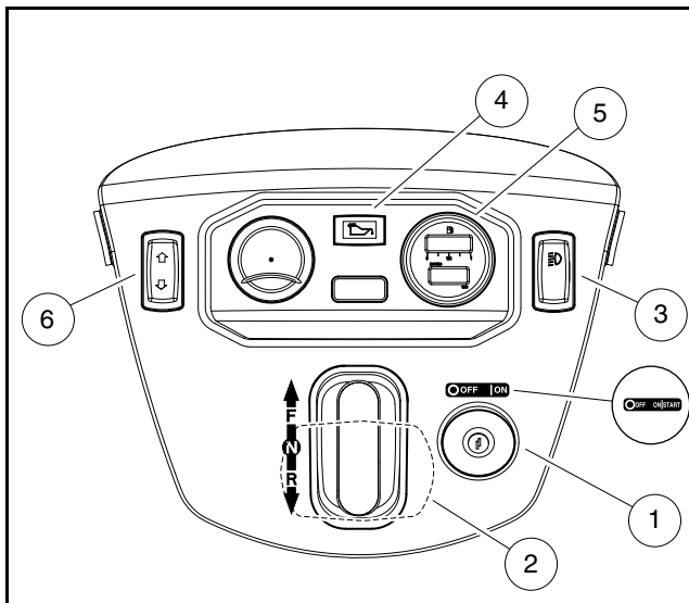
Figure 6 Instrument Panel
