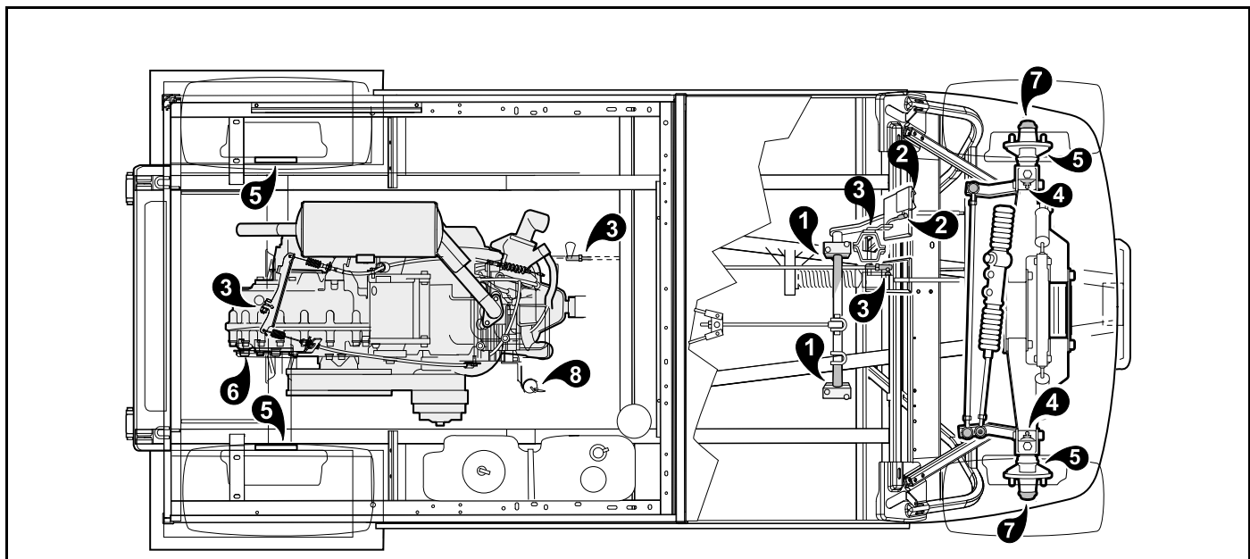
2823 Figure 15 Lubrication Points
