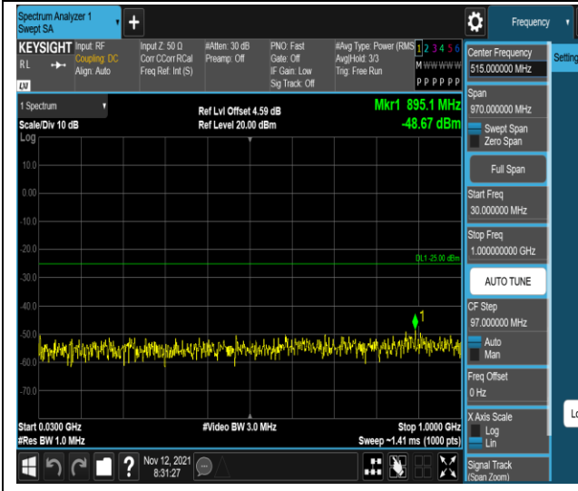
Band38-5MHz-QPSK-37775-1 RB#0-Range 1:30~1000MHz
