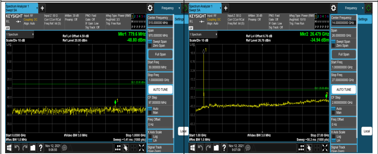
Band38-5MHz-16QAM-38225-1 RB#0-Range 1:30~1000MHz
