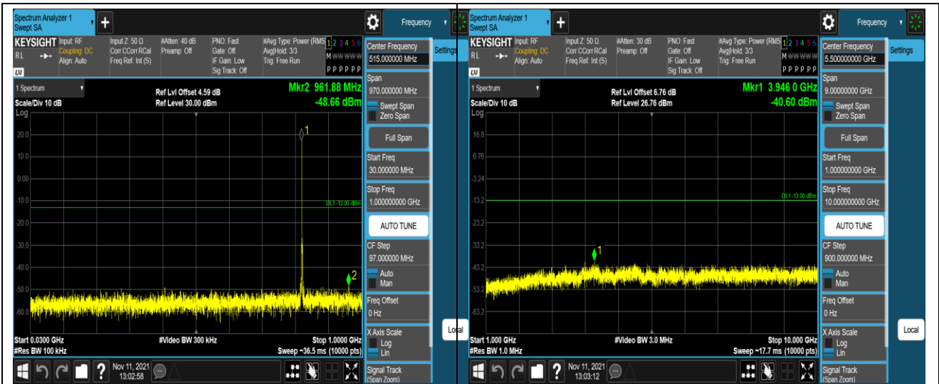
Band5-1.4MHz-16QAM-20407-1RB#0-Range 1:30~1000MHz
