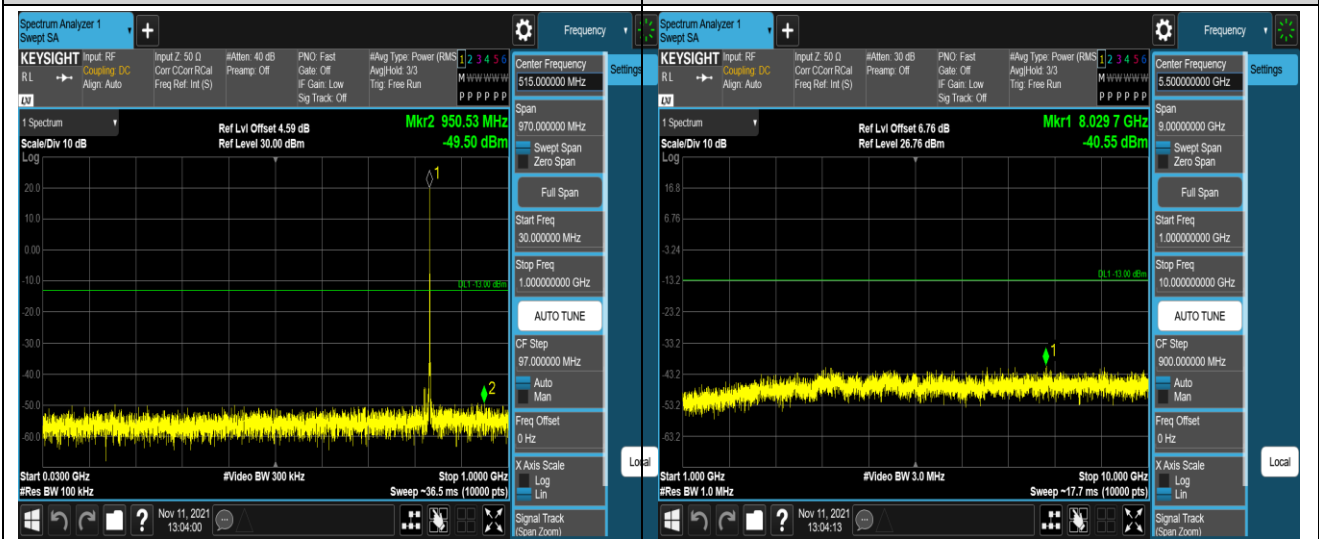
Band5-1.4MHz-16QAM-20525-1RB#0-Range 1:30~1000MHz
