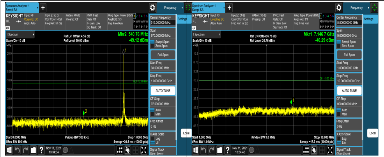
Band5-10MHz-16QAM-20450-1 RB#0-Range 1:30~1000MHz Band5-10MHz-16QAM-20450-1 RB#0-Range 2: 1000~10000MHz
