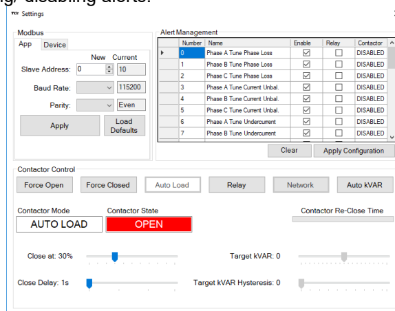
Figure 7: PQvision Settings
