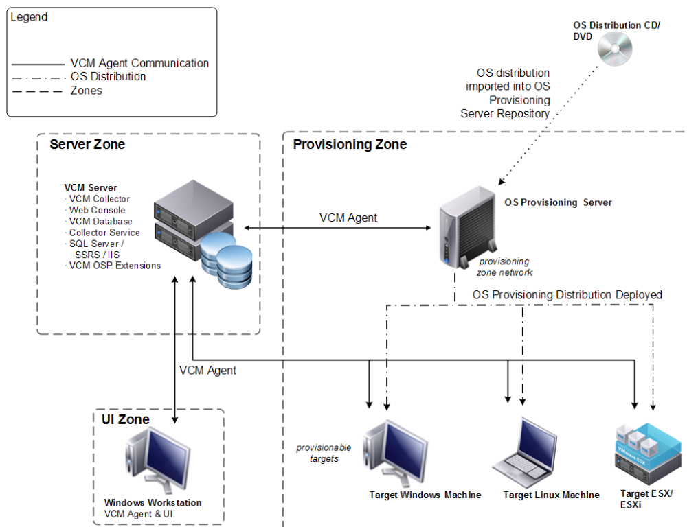
Figure 11-1. Operating System Provisioning Components
