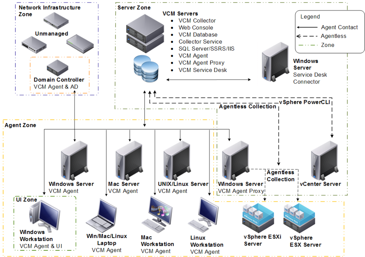
Figure 1–1. VCM Components and Zones
