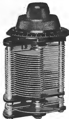
UNITED VERNIER CONDENSER.
