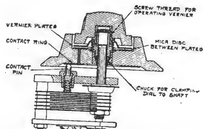
UNITED SELF-CONTAINED VERNIER DIAL.
